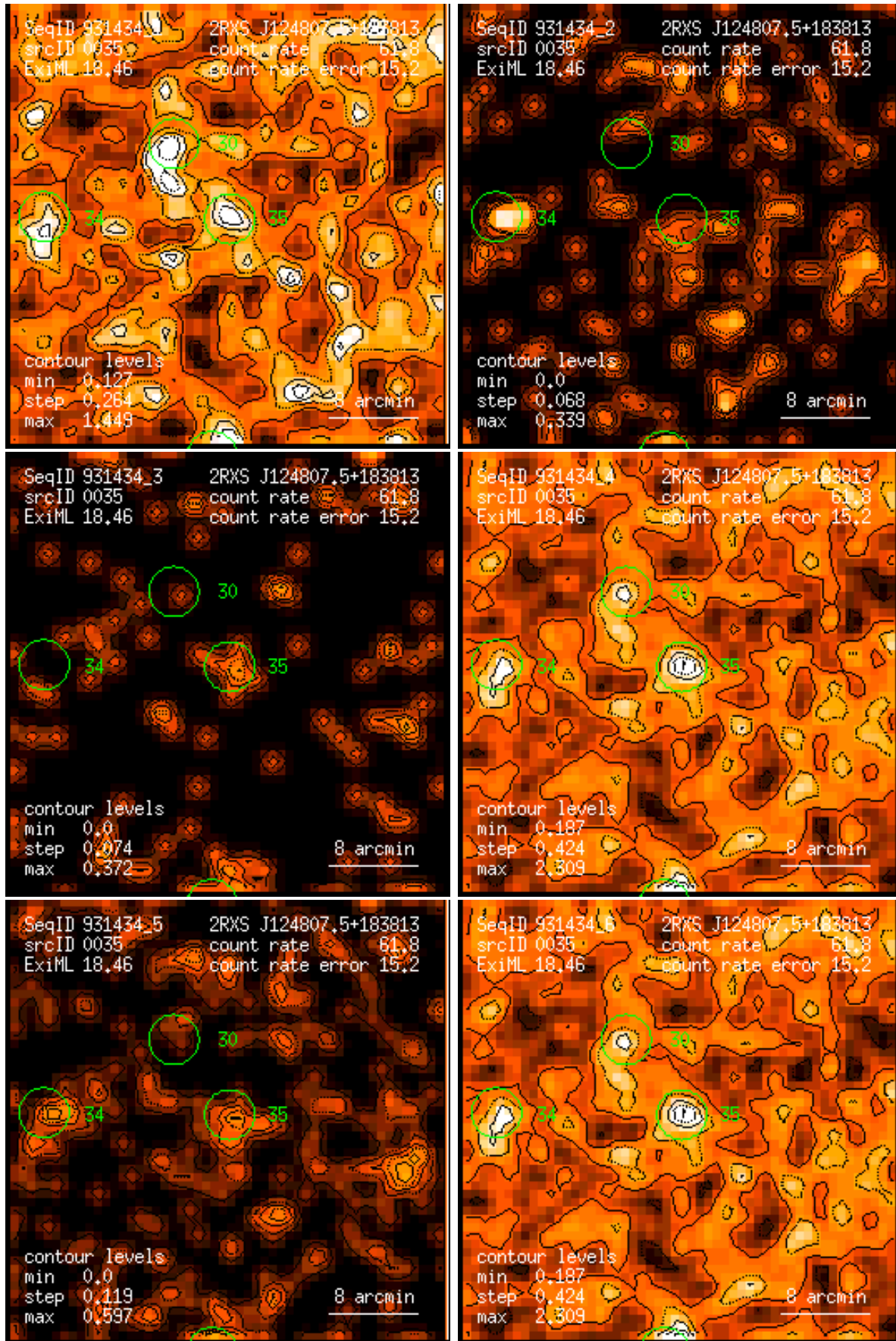
Figure 35: RASS 931434: detection 0035: band rate images, Gaussian filter: (1) PSPC channels 11 – 41, (2) 52 – 90, (3) 91 – 201, (4) 11 – 235, (5) 52 – 201, (6) 11 – 201. Broad band rates in counts/ks. Band rate contour levels in counts/ks/arcmin 2 .
