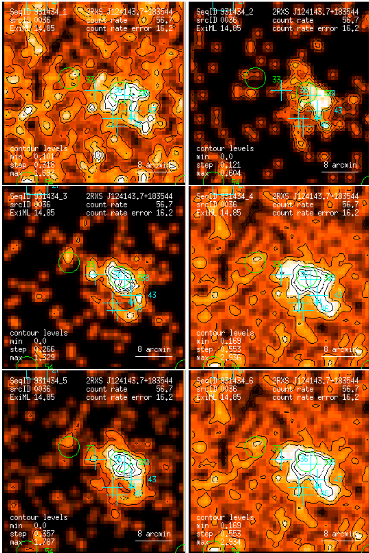
Figure 36: RASS 931434: detection 0036: band rate images, Gaussian filter: (1) PSPC channels 11 – 41, (2) 52 – 90, (3) 91 – 201, (4) 11 – 235, (5) 52 – 201, (6) 11 – 201. Broad band rates in counts/ks. Band rate contour levels in counts/ks/arcmin 2 .
