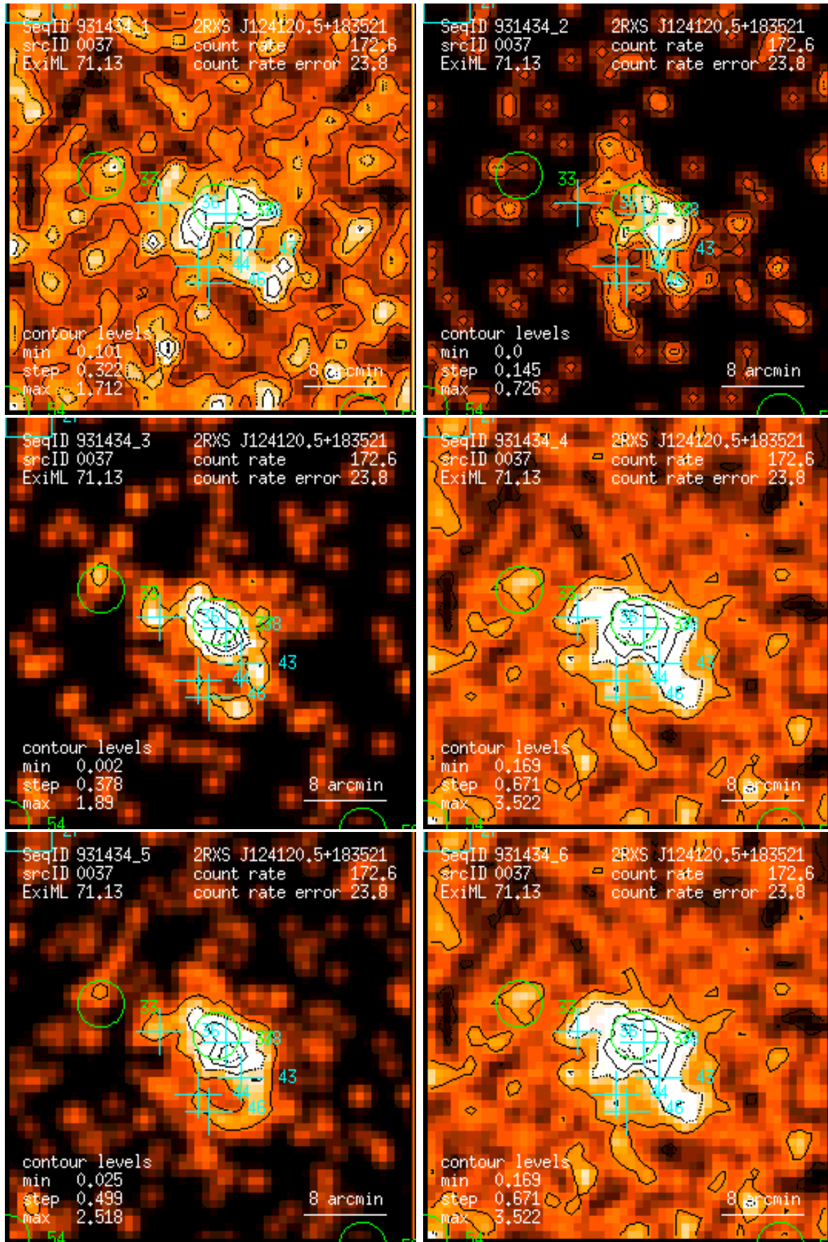
Figure 37: RASS 931434: detection 0037: band rate images, Gaussian filter: (1) PSPC channels 11 – 41, (2) 52 – 90, (3) 91 – 201, (4) 11 – 235, (5) 52 – 201, (6) 11 – 201. Broad band rates in counts/ks. Band rate contour levels in counts/ks/arcmin 2 .
