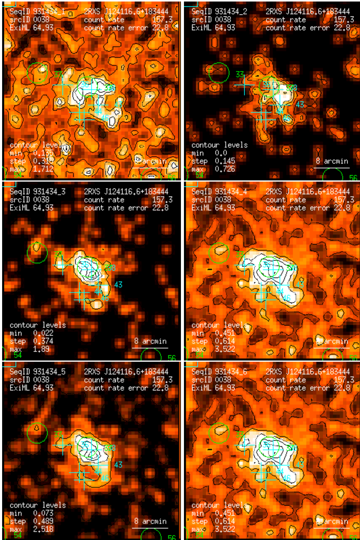
Figure 38: RASS 931434: detection 0038: band rate images, Gaussian filter: (1) PSPC channels 11 – 41, (2) 52 – 90, (3) 91 – 201, (4) 11 – 235, (5) 52 – 201, (6) 11 – 201. Broad band rates in counts/ks. Band rate contour levels in counts/ks/arcmin 2 .
