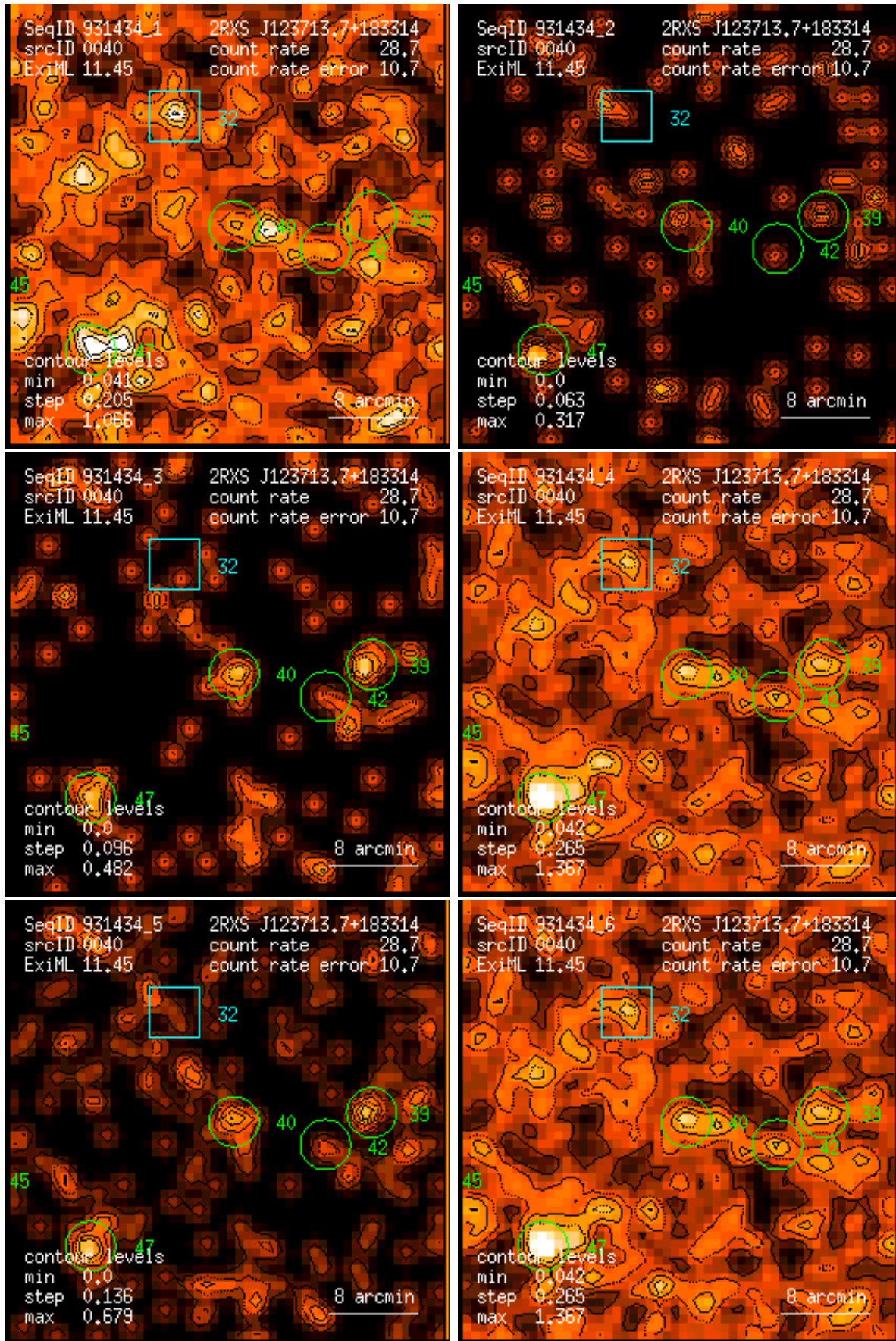
Figure 40: RASS 931434: detection 0040: band rate images, Gaussian filter: (1) PSPC channels 11 – 41, (2) 52 – 90, (3) 91 – 201, (4) 11 – 235, (5) 52 – 201, (6) 11 – 201. Broad band rates in counts/ks. Band rate contour levels in counts/ks/arcmin 2 .
