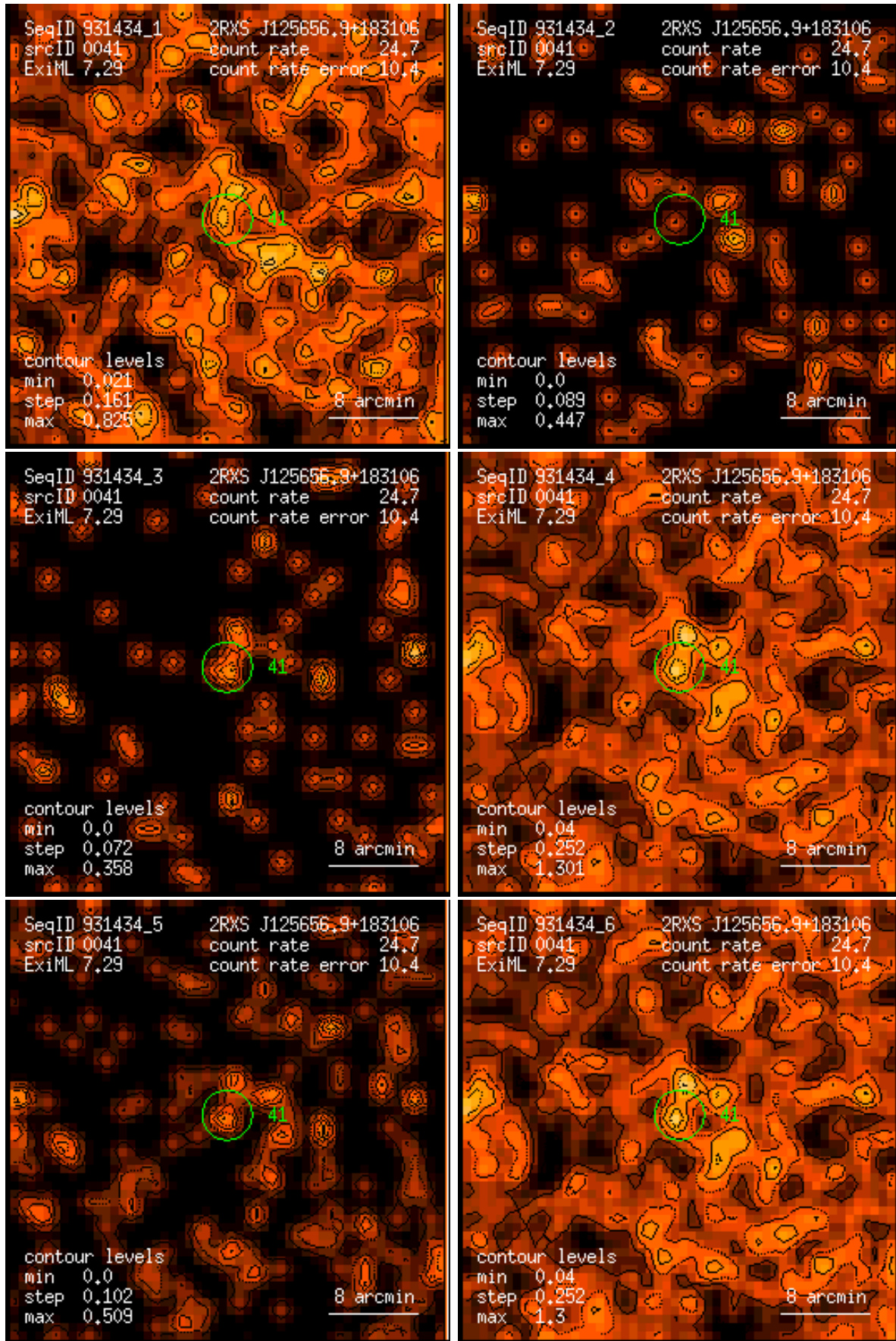
Figure 41: RASS 931434: detection 0041: band rate images, Gaussian filter: (1) PSPC channels 11 – 41, (2) 52 – 90, (3) 91 – 201, (4) 11 – 235, (5) 52 – 201, (6) 11 – 201. Broad band rates in counts/ks. Band rate contour levels in counts/ks/arcmin 2 .
