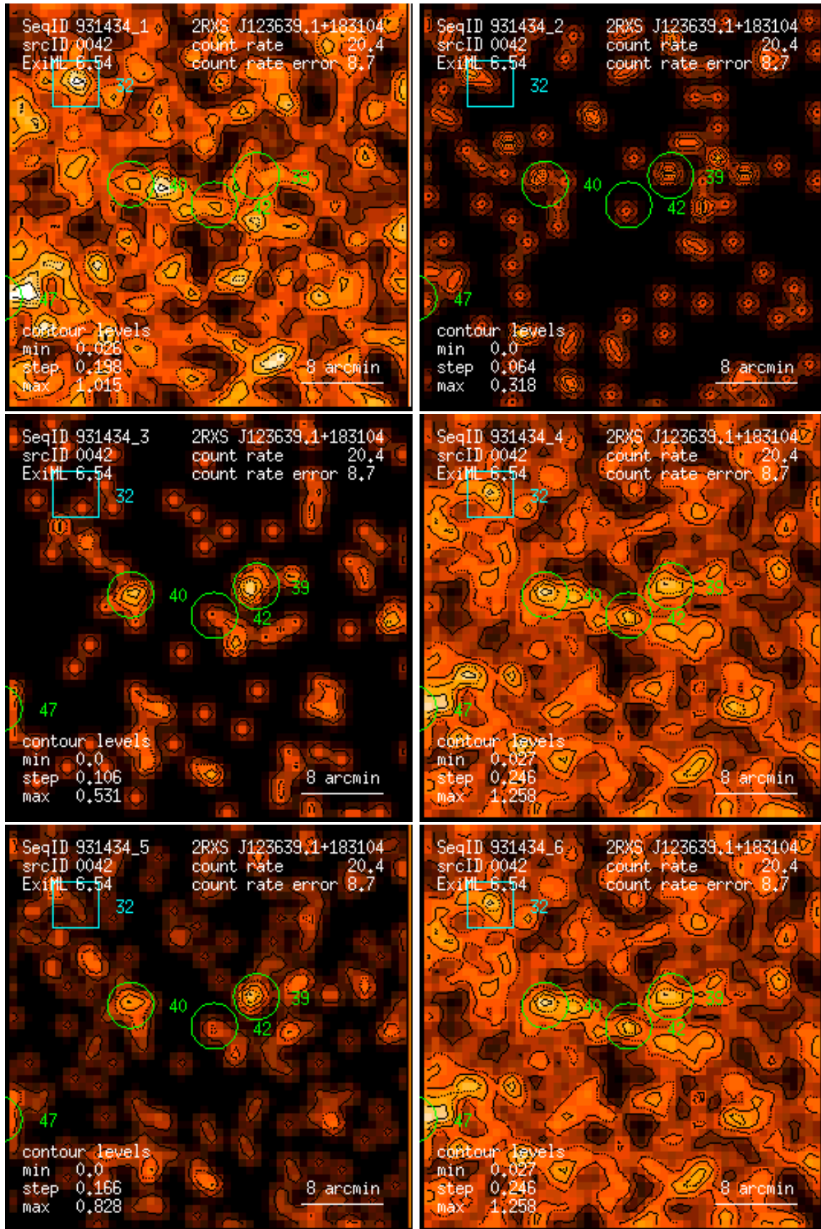
Figure 42: RASS 931434: detection 0042: band rate images, Gaussian filter: (1) PSPC channels 11 – 41, (2) 52 – 90, (3) 91 – 201, (4) 11 – 235, (5) 52 – 201, (6) 11 – 201. Broad band rates in counts/ks. Band rate contour levels in counts/ks/arcmin 2 .
