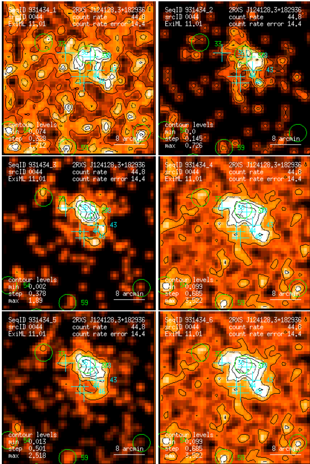
Figure 44: RASS 931434: detection 0044: band rate images, Gaussian filter: (1) PSPC channels 11 – 41, (2) 52 – 90, (3) 91 – 201, (4) 11 – 235, (5) 52 – 201, (6) 11 – 201. Broad band rates in counts/ks. Band rate contour levels in counts/ks/arcmin 2 .
