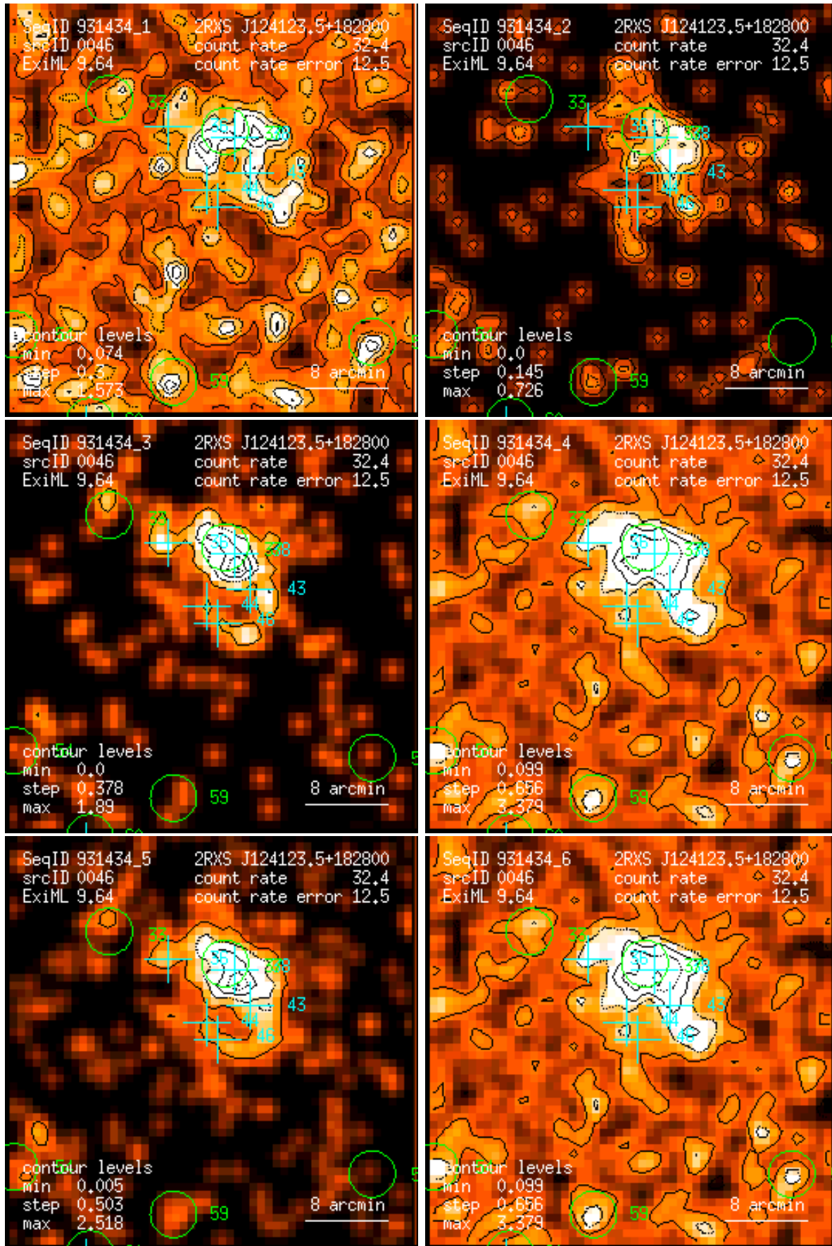
Figure 46: RASS 931434: detection 0046: band rate images, Gaussian filter: (1) PSPC channels 11 – 41, (2) 52 – 90, (3) 91 – 201, (4) 11 – 235, (5) 52 – 201, (6) 11 – 201. Broad band rates in counts/ks. Band rate contour levels in counts/ks/arcmin 2 .
