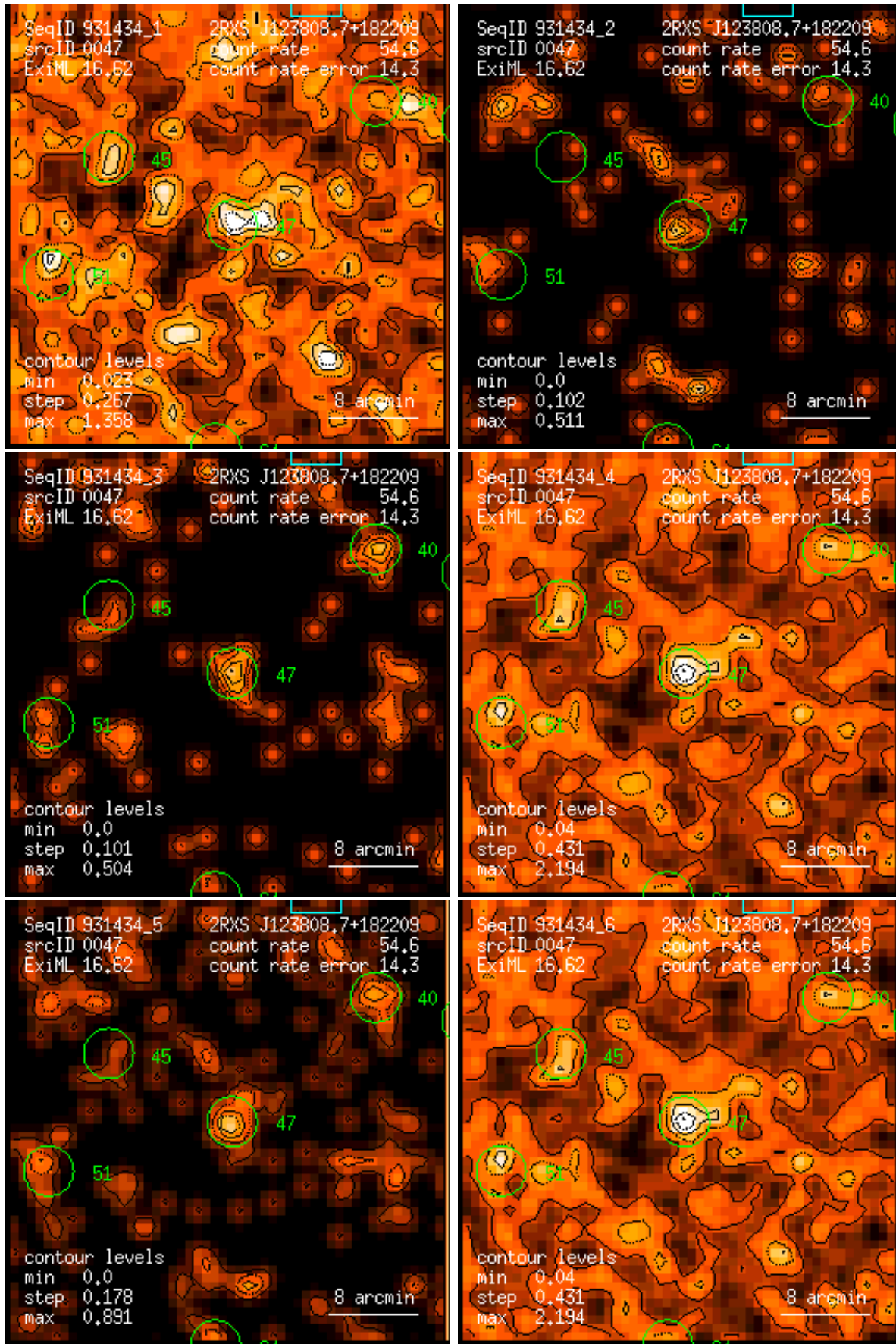
Figure 47: RASS 931434: detection 0047: band rate images, Gaussian filter: (1) PSPC channels 11 – 41, (2) 52 – 90, (3) 91 – 201, (4) 11 – 235, (5) 52 – 201, (6) 11 – 201. Broad band rates in counts/ks. Band rate contour levels in counts/ks/arcmin 2 .
