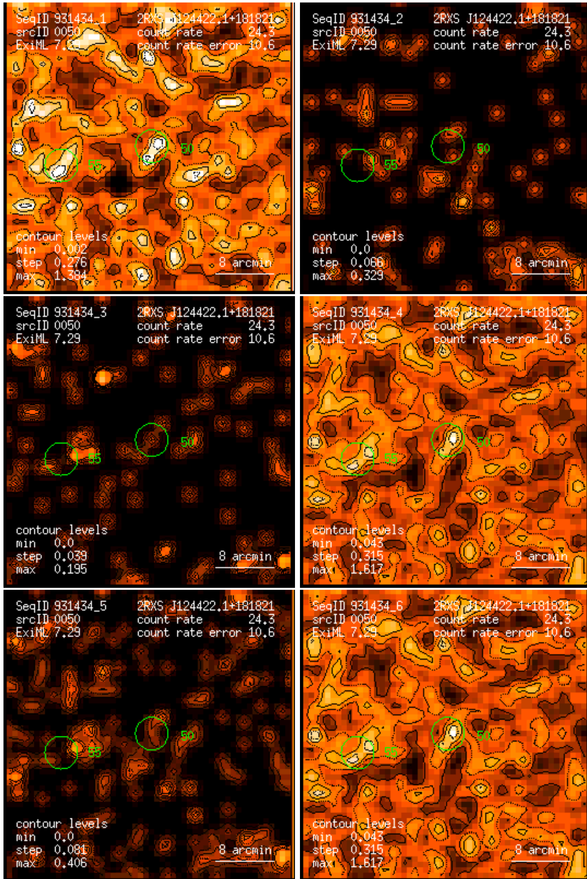
Figure 50: RASS 931434: detection 0050: band rate images, Gaussian filter: (1) PSPC channels 11 – 41, (2) 52 – 90, (3) 91 – 201, (4) 11 – 235, (5) 52 – 201, (6) 11 – 201. Broad band rates in counts/ks. Band rate contour levels in counts/ks/arcmin 2 .
