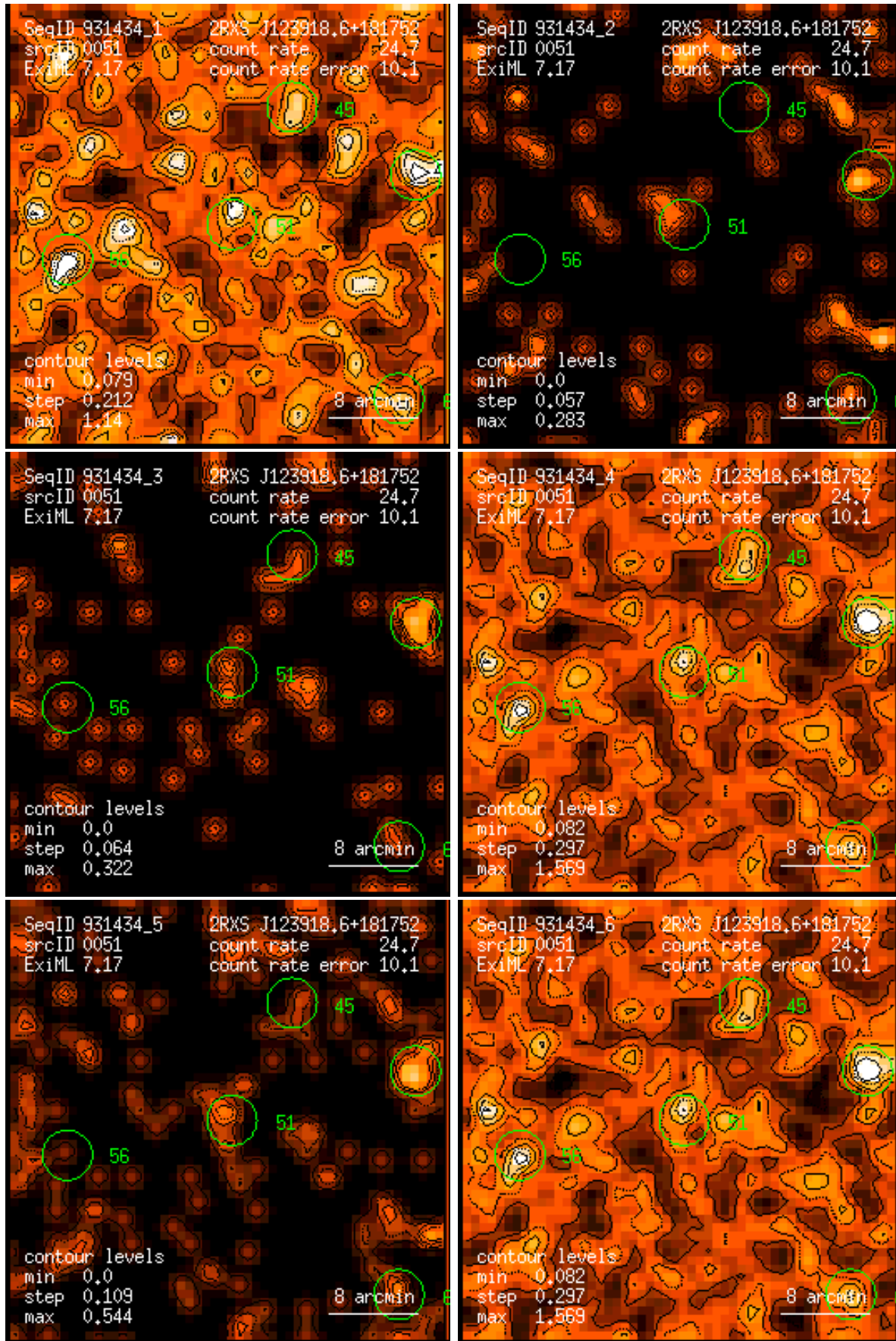
Figure 51: RASS 931434: detection 0051: band rate images, Gaussian filter: (1) PSPC channels 11 – 41, (2) 52 – 90, (3) 91 – 201, (4) 11 – 235, (5) 52 – 201, (6) 11 – 201. Broad band rates in counts/ks. Band rate contour levels in counts/ks/arcmin 2 .
