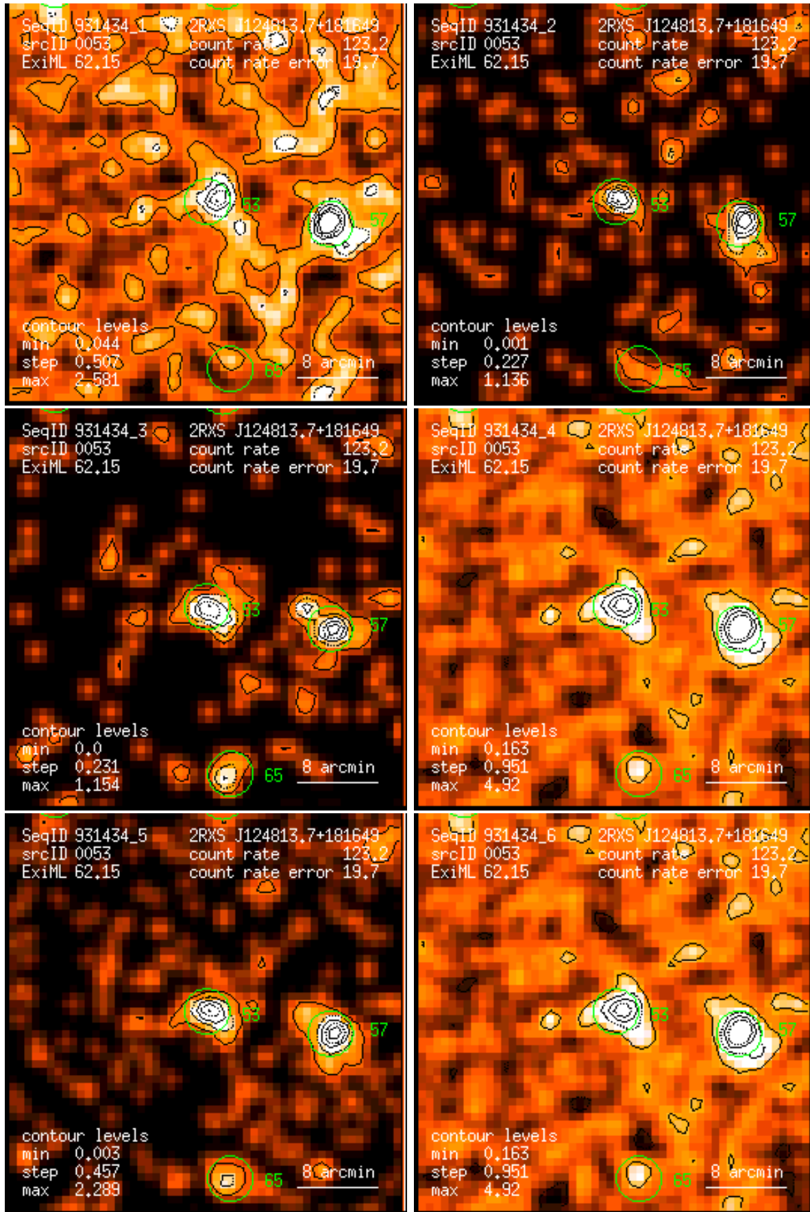
Figure 53: RASS 931434: detection 0053: band rate images, Gaussian filter: (1) PSPC channels 11 – 41, (2) 52 – 90, (3) 91 – 201, (4) 11 – 235, (5) 52 – 201, (6) 11 – 201. Broad band rates in counts/ks. Band rate contour levels in counts/ks/arcmin 2 .
