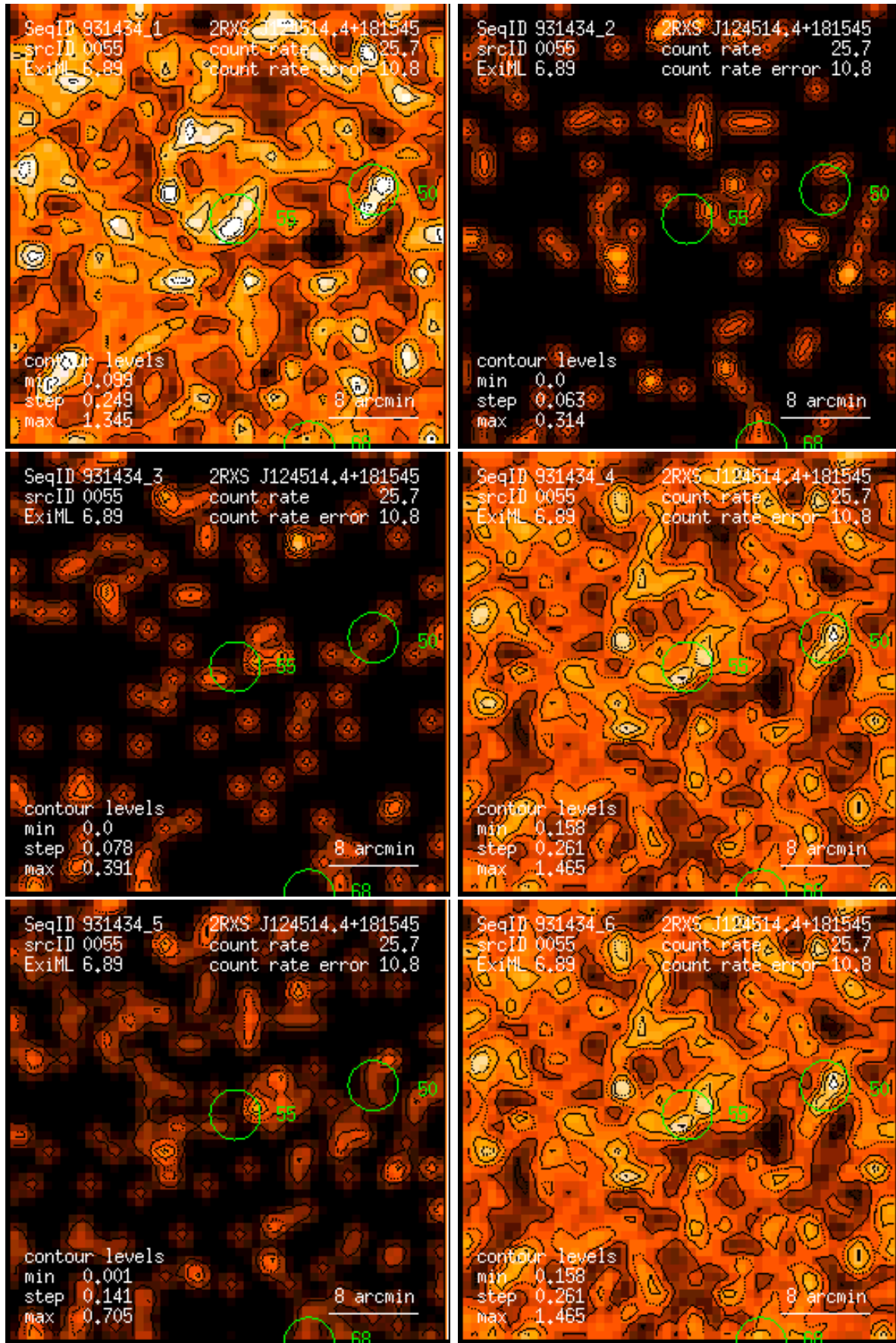
Figure 55: RASS 931434: detection 0055: band rate images, Gaussian filter: (1) PSPC channels 11 – 41, (2) 52 – 90, (3) 91 – 201, (4) 11 – 235, (5) 52 – 201, (6) 11 – 201. Broad band rates in counts/ks. Band rate contour levels in counts/ks/arcmin 2 .
