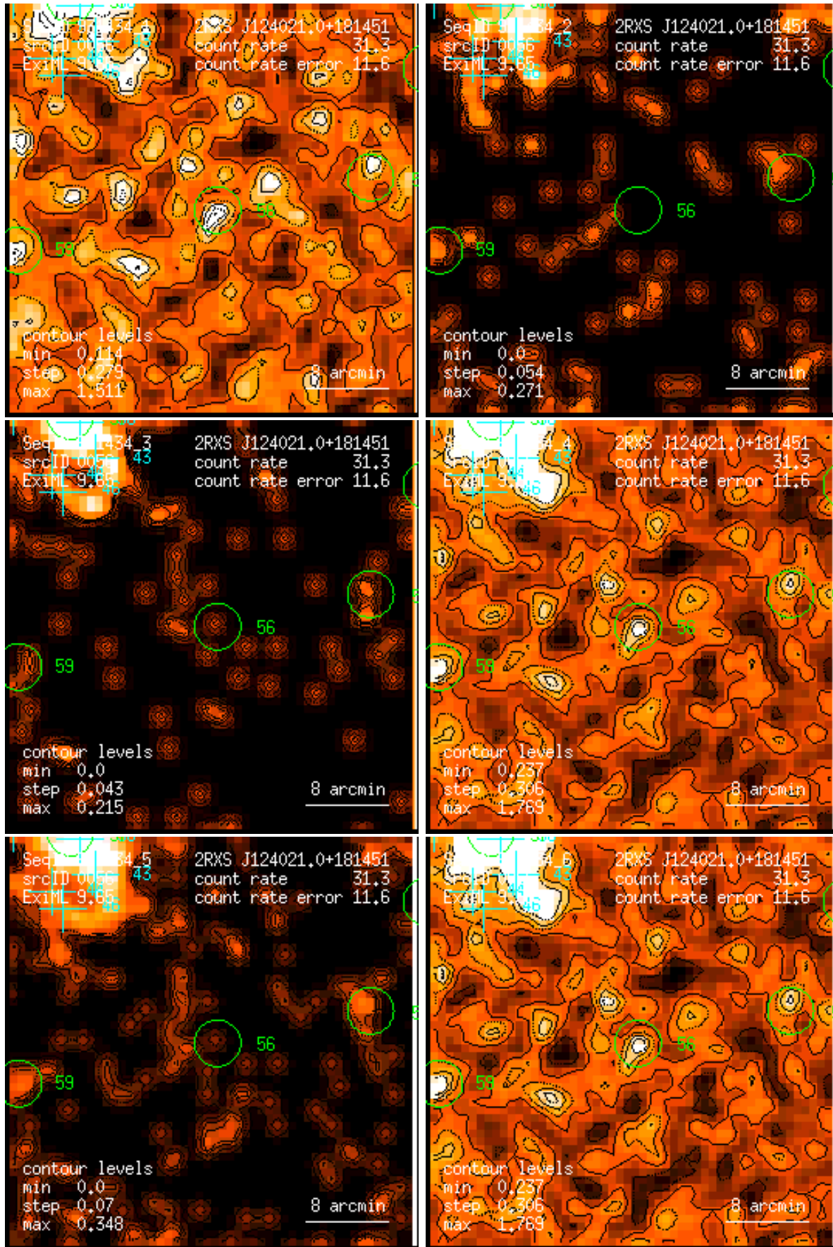
Figure 56: RASS 931434: detection 0056: band rate images, Gaussian filter: (1) PSPC channels 11 – 41, (2) 52 – 90, (3) 91 – 201, (4) 11 – 235, (5) 52 – 201, (6) 11 – 201. Broad band rates in counts/ks. Band rate contour levels in counts/ks/arcmin 2 .
