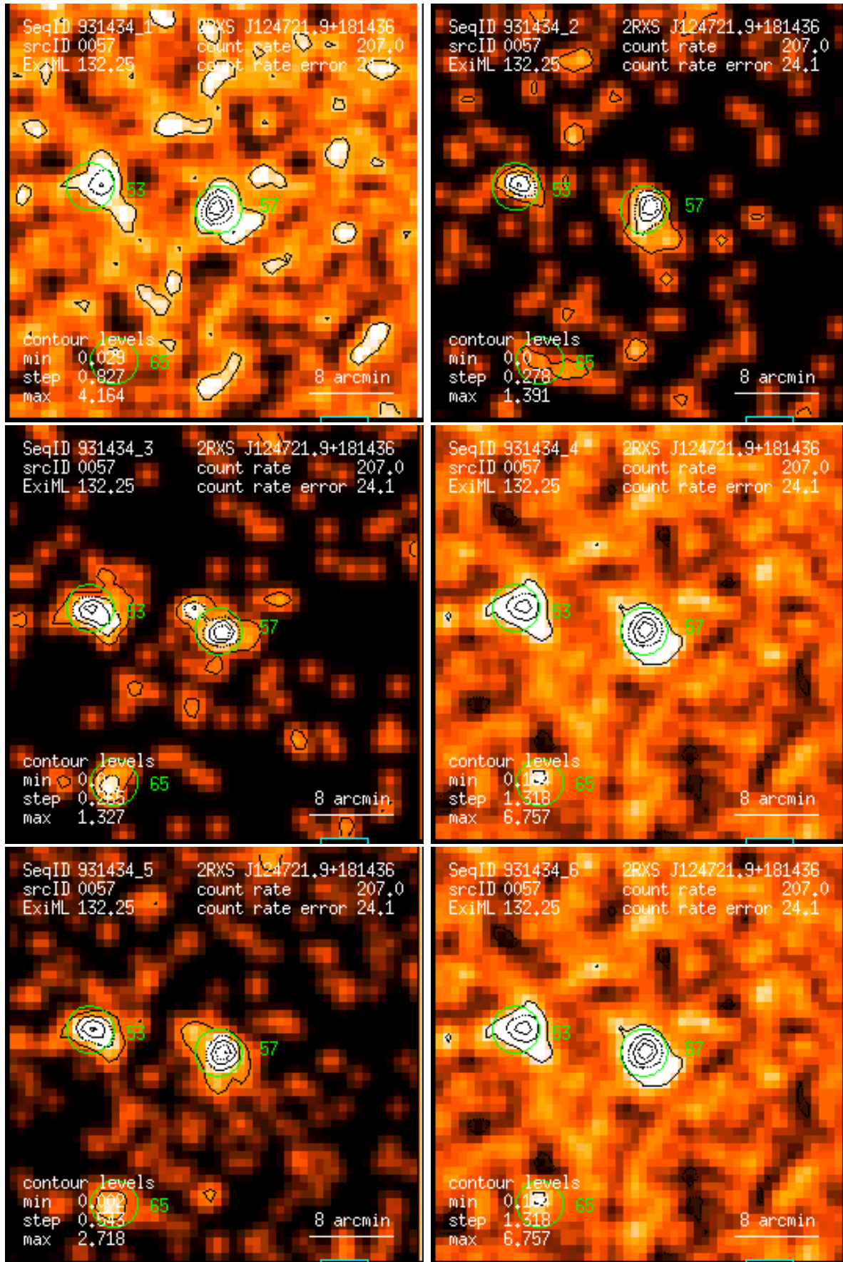
Figure 57: RASS 931434: detection 0057: band rate images, Gaussian filter: (1) PSPC channels 11 – 41, (2) 52 – 90, (3) 91 – 201, (4) 11 – 235, (5) 52 – 201, (6) 11 – 201. Broad band rates in counts/ks. Band rate contour levels in counts/ks/arcmin 2 .
