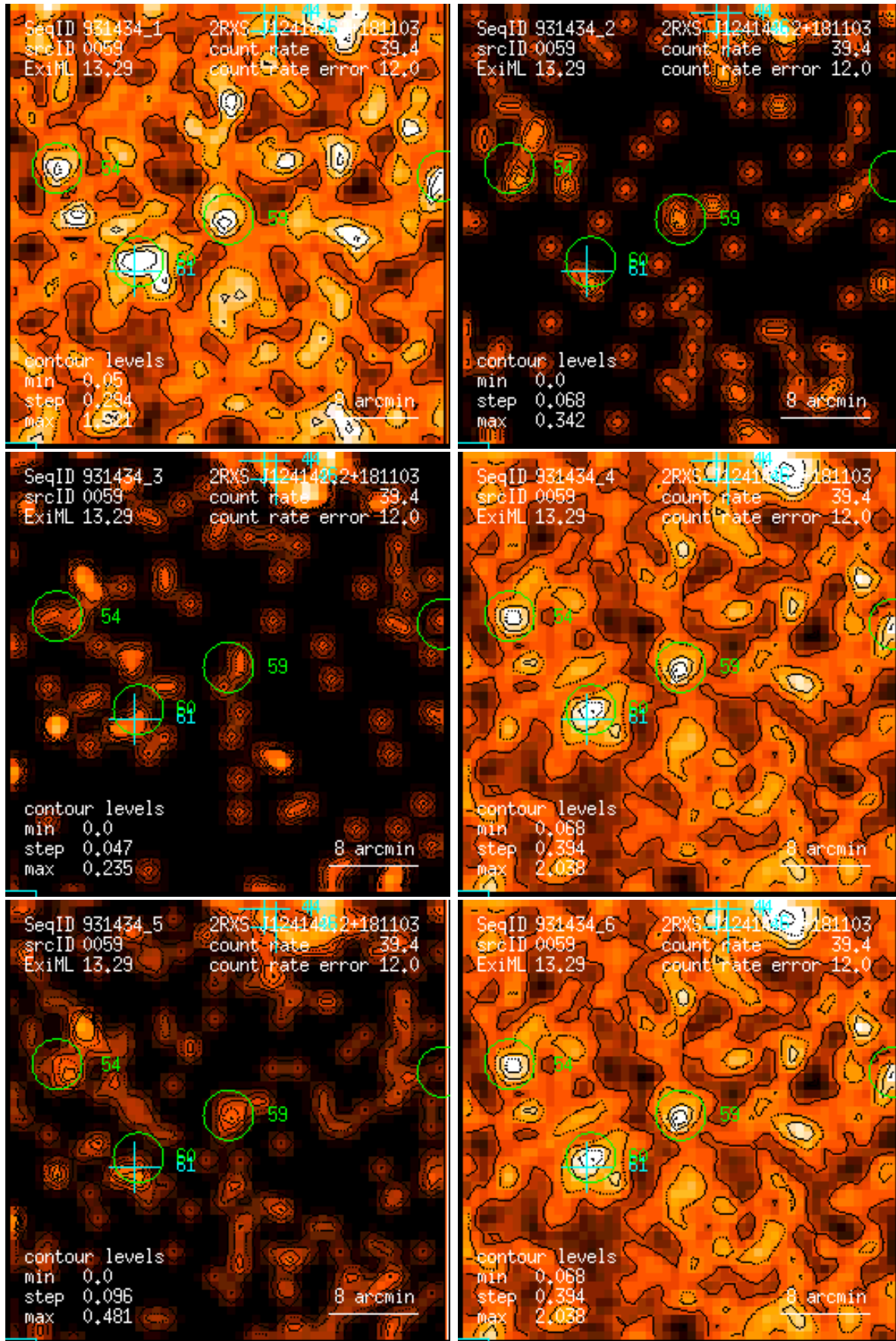
Figure 59: RASS 931434: detection 0059: band rate images, Gaussian filter: (1) PSPC channels 11 – 41, (2) 52 – 90, (3) 91 – 201, (4) 11 – 235, (5) 52 – 201, (6) 11 – 201. Broad band rates in counts/ks. Band rate contour levels in counts/ks/arcmin 2 .
