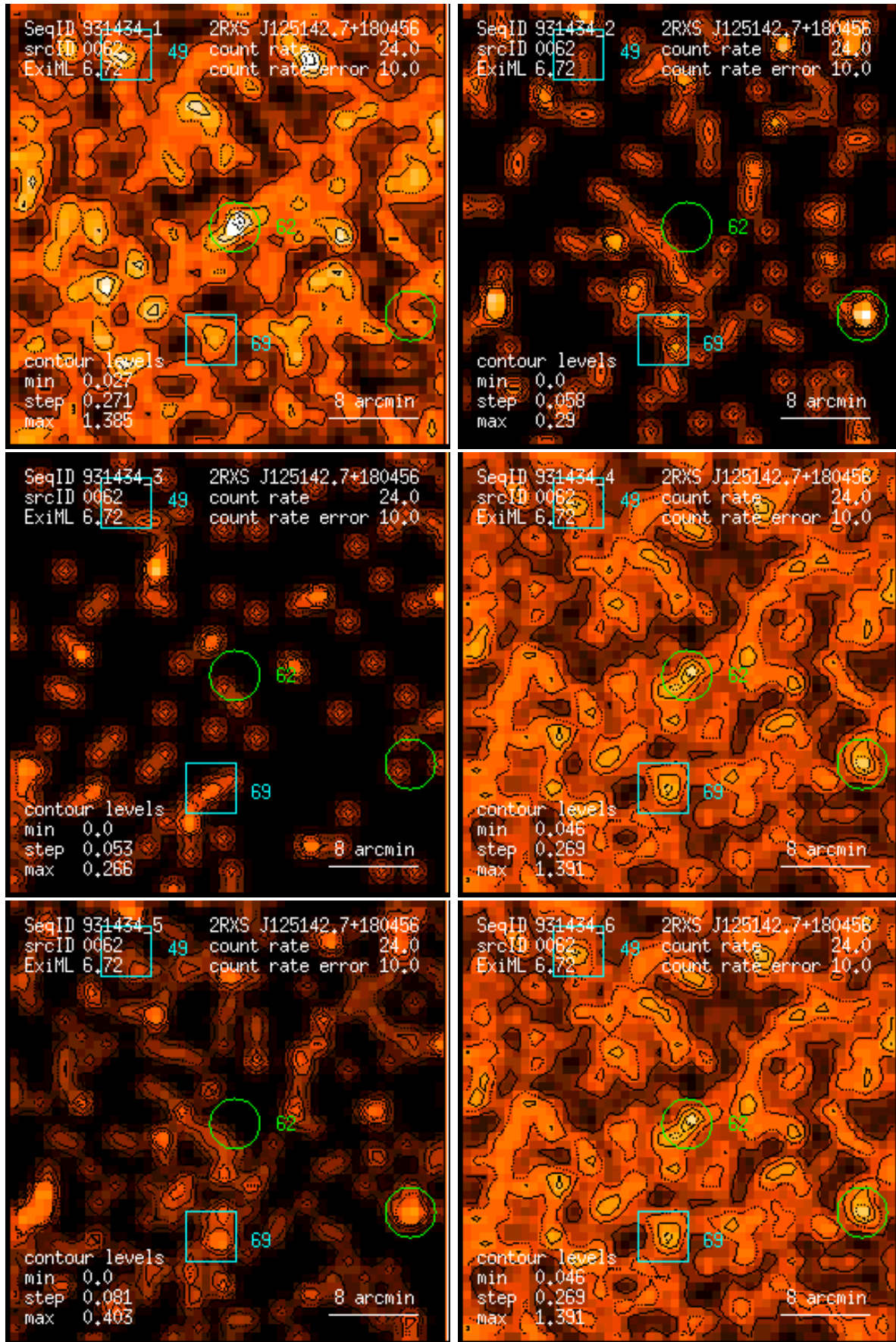
Figure 62: RASS 931434: detection 0062: band rate images, Gaussian filter: (1) PSPC channels 11 – 41, (2) 52 – 90, (3) 91 – 201, (4) 11 – 235, (5) 52 – 201, (6) 11 – 201. Broad band rates in counts/ks. Band rate contour levels in counts/ks/arcmin 2 .
