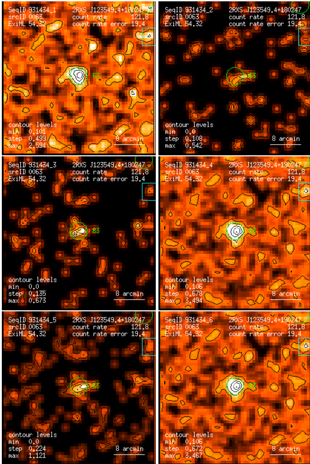
Figure 63: RASS 931434: detection 0063: band rate images, Gaussian filter: (1) PSPC channels 11 – 41, (2) 52 – 90, (3) 91 – 201, (4) 11 – 235, (5) 52 – 201, (6) 11 – 201. Broad band rates in counts/ks. Band rate contour levels in counts/ks/arcmin 2 .
