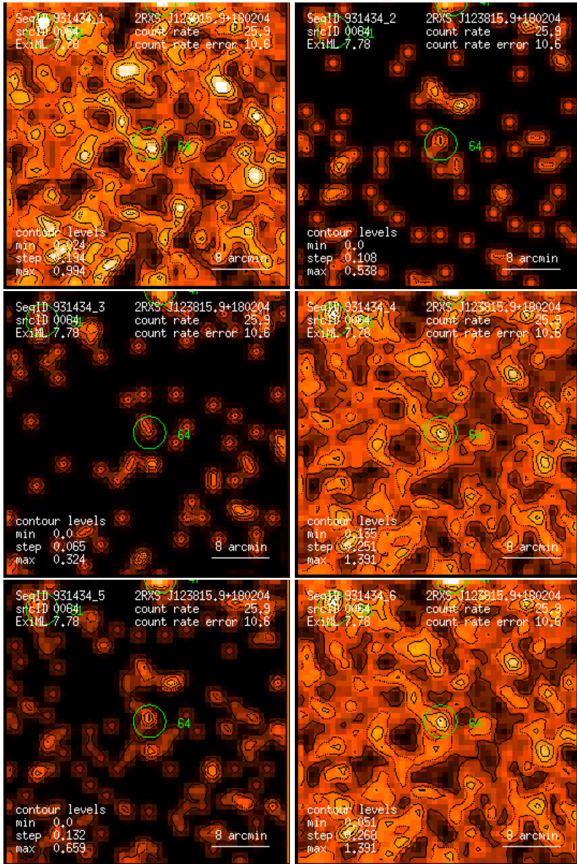
Figure 64: RASS 931434: detection 0064: band rate images, Gaussian filter: (1) PSPC channels 11 – 41, (2) 52 – 90, (3) 91 – 201, (4) 11 – 235, (5) 52 – 201, (6) 11 – 201. Broad band rates in counts/ks. Band rate contour levels in counts/ks/arcmin 2 .
