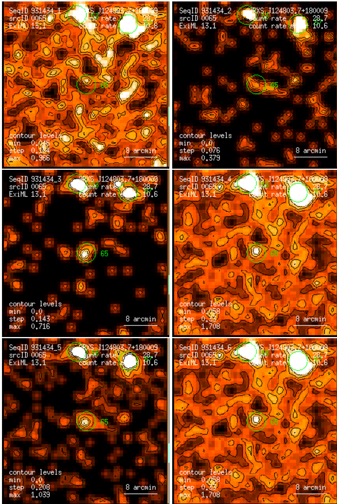
Figure 65: RASS 931434: detection 0065: band rate images, Gaussian filter: (1) PSPC channels 11 – 41, (2) 52 – 90, (3) 91 – 201, (4) 11 – 235, (5) 52 – 201, (6) 11 – 201. Broad band rates in counts/ks. Band rate contour levels in counts/ks/arcmin 2 .
