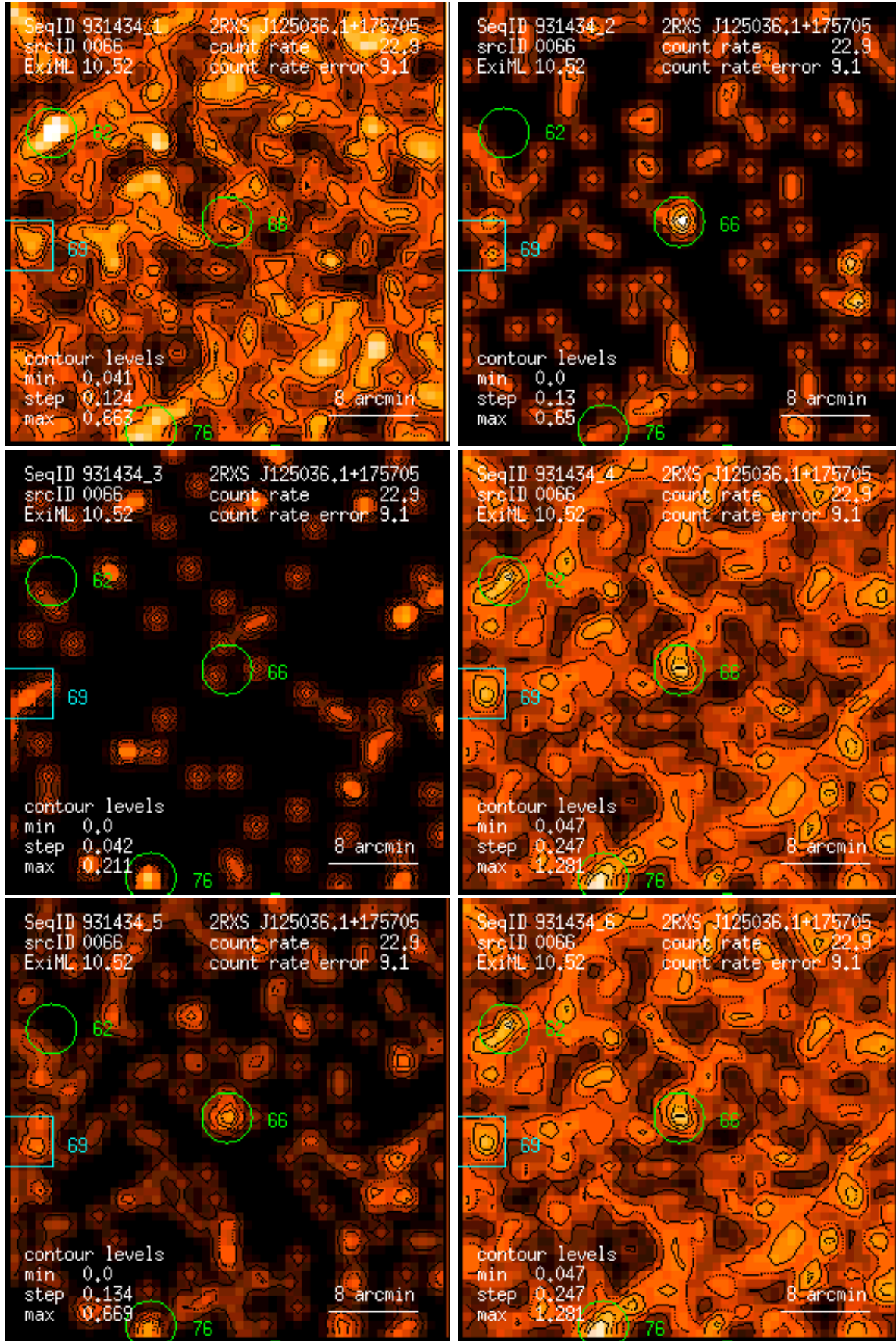
Figure 66: RASS 931434: detection 0066: band rate images, Gaussian filter: (1) PSPC channels 11 – 41, (2) 52 – 90, (3) 91 – 201, (4) 11 – 235, (5) 52 – 201, (6) 11 – 201. Broad band rates in counts/ks. Band rate contour levels in counts/ks/arcmin 2 .
