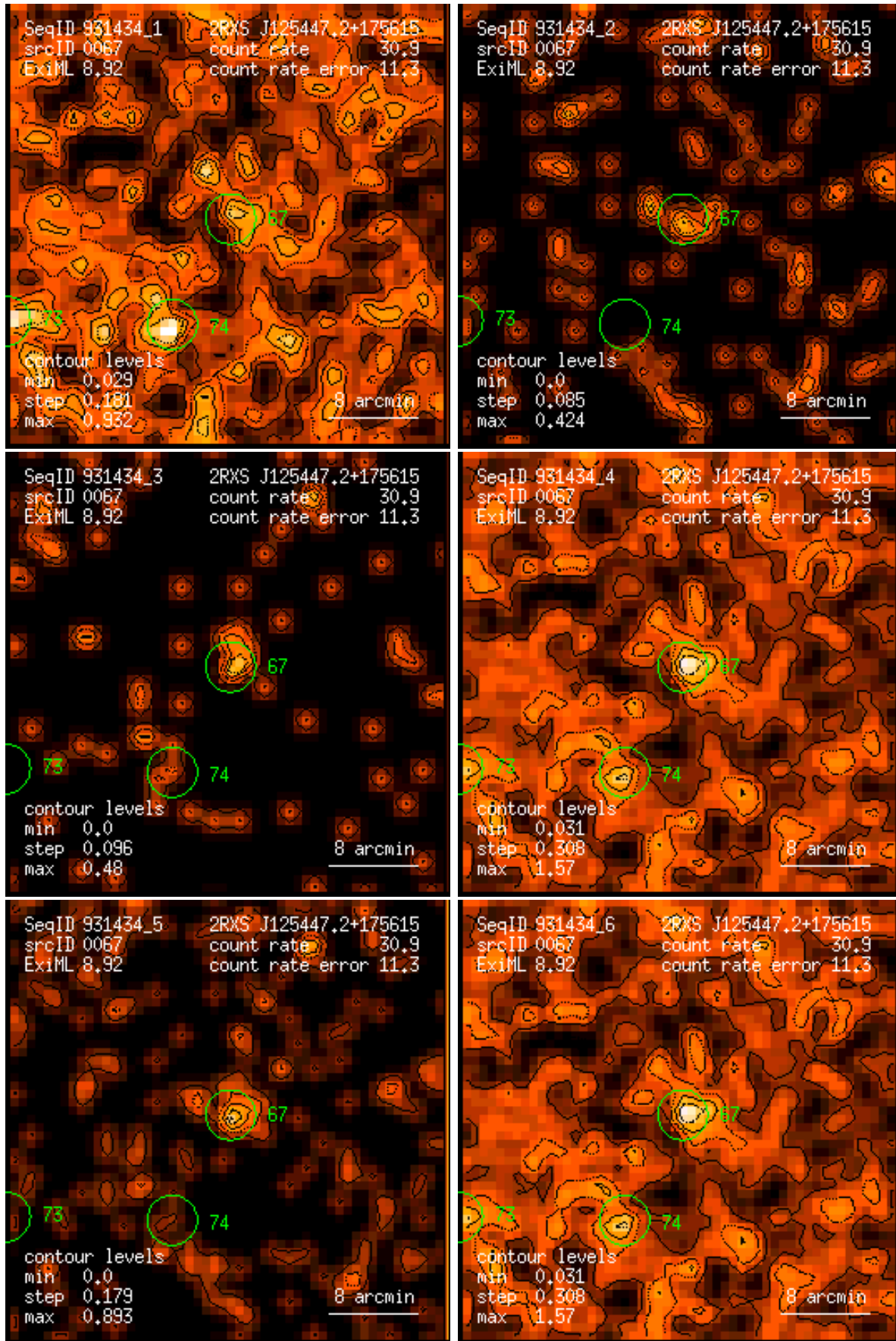
Figure 67: RASS 931434: detection 0067: band rate images, Gaussian filter: (1) PSPC channels 11 – 41, (2) 52 – 90, (3) 91 – 201, (4) 11 – 235, (5) 52 – 201, (6) 11 – 201. Broad band rates in counts/ks. Band rate contour levels in counts/ks/arcmin 2 .
