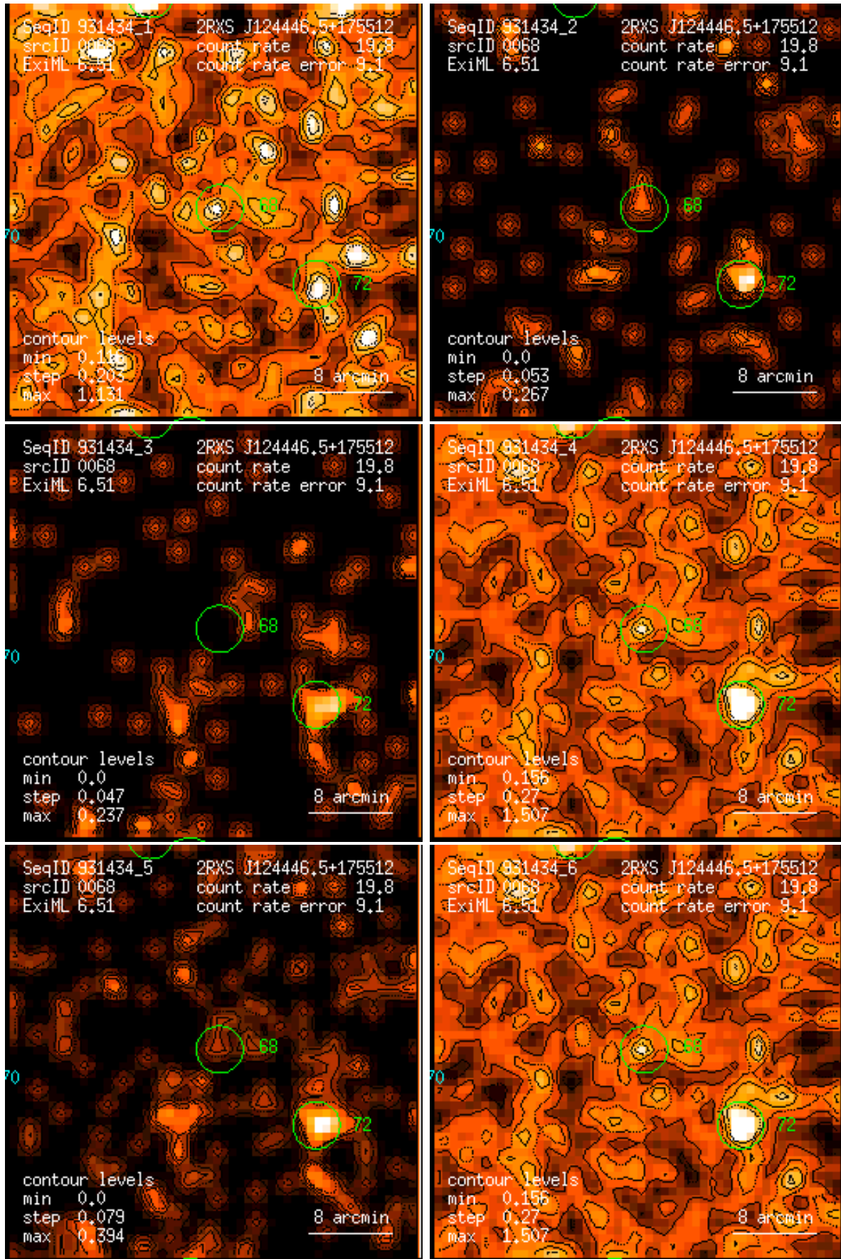
Figure 68: RASS 931434: detection 0068: band rate images, Gaussian filter: (1) PSPC channels 11 – 41, (2) 52 – 90, (3) 91 – 201, (4) 11 – 235, (5) 52 – 201, (6) 11 – 201. Broad band rates in counts/ks. Band rate contour levels in counts/ks/arcmin 2 .
