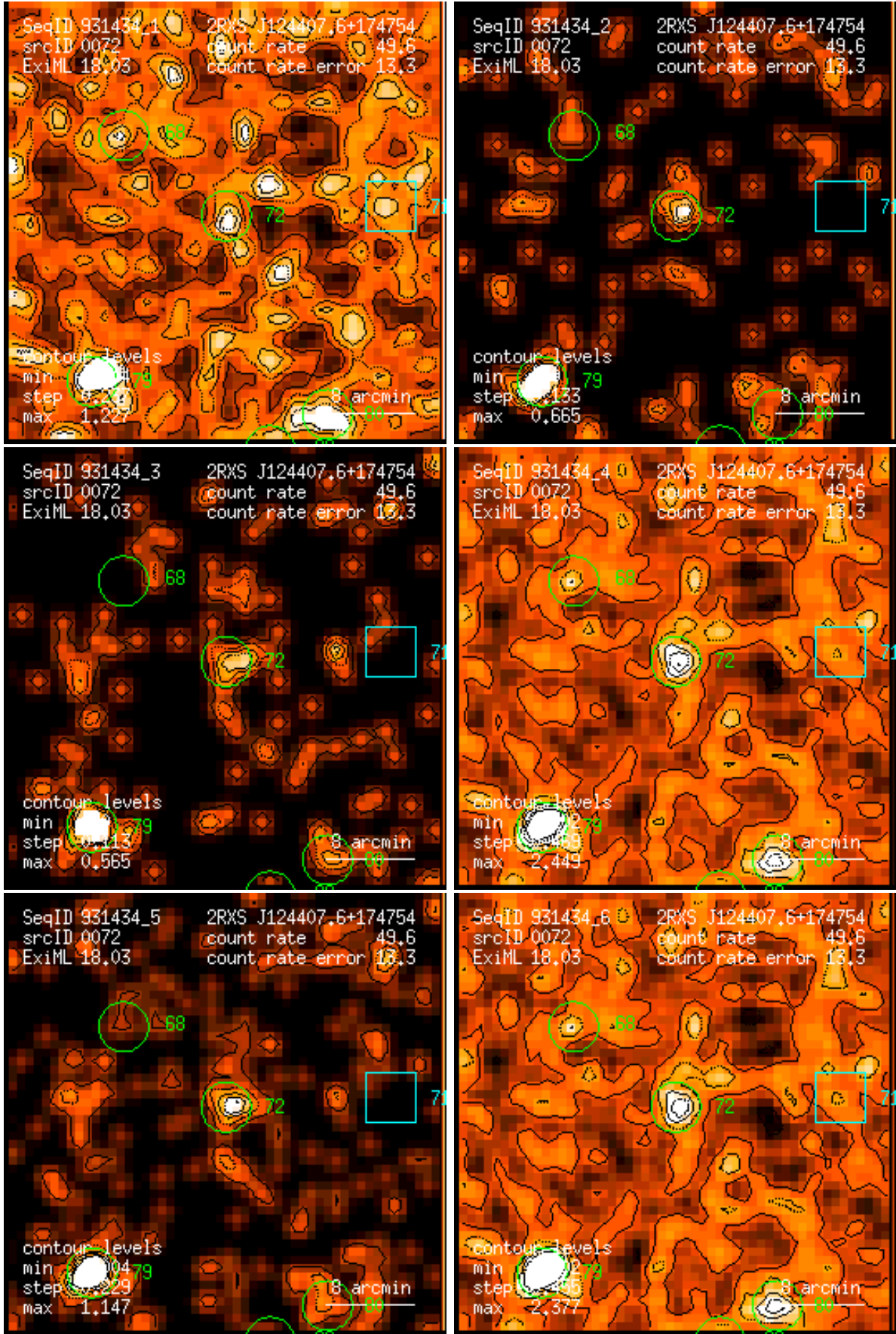
Figure 72: RASS 931434: detection 0072: band rate images, Gaussian filter: (1) PSPC channels 11 – 41, (2) 52 – 90, (3) 91 – 201, (4) 11 – 235, (5) 52 – 201, (6) 11 – 201. Broad band rates in counts/ks. Band rate contour levels in counts/ks/arcmin 2 .
