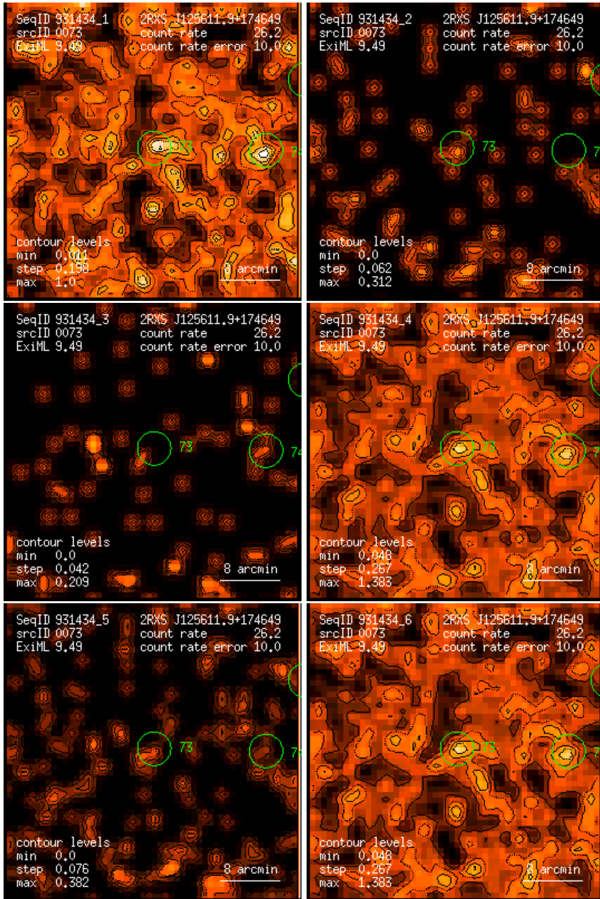
Figure 73: RASS 931434: detection 0073: band rate images, Gaussian filter: (1) PSPC channels 11 – 41, (2) 52 – 90, (3) 91 – 201, (4) 11 – 235, (5) 52 – 201, (6) 11 – 201. Broad band rates in counts/ks. Band rate contour levels in counts/ks/arcmin 2 .
