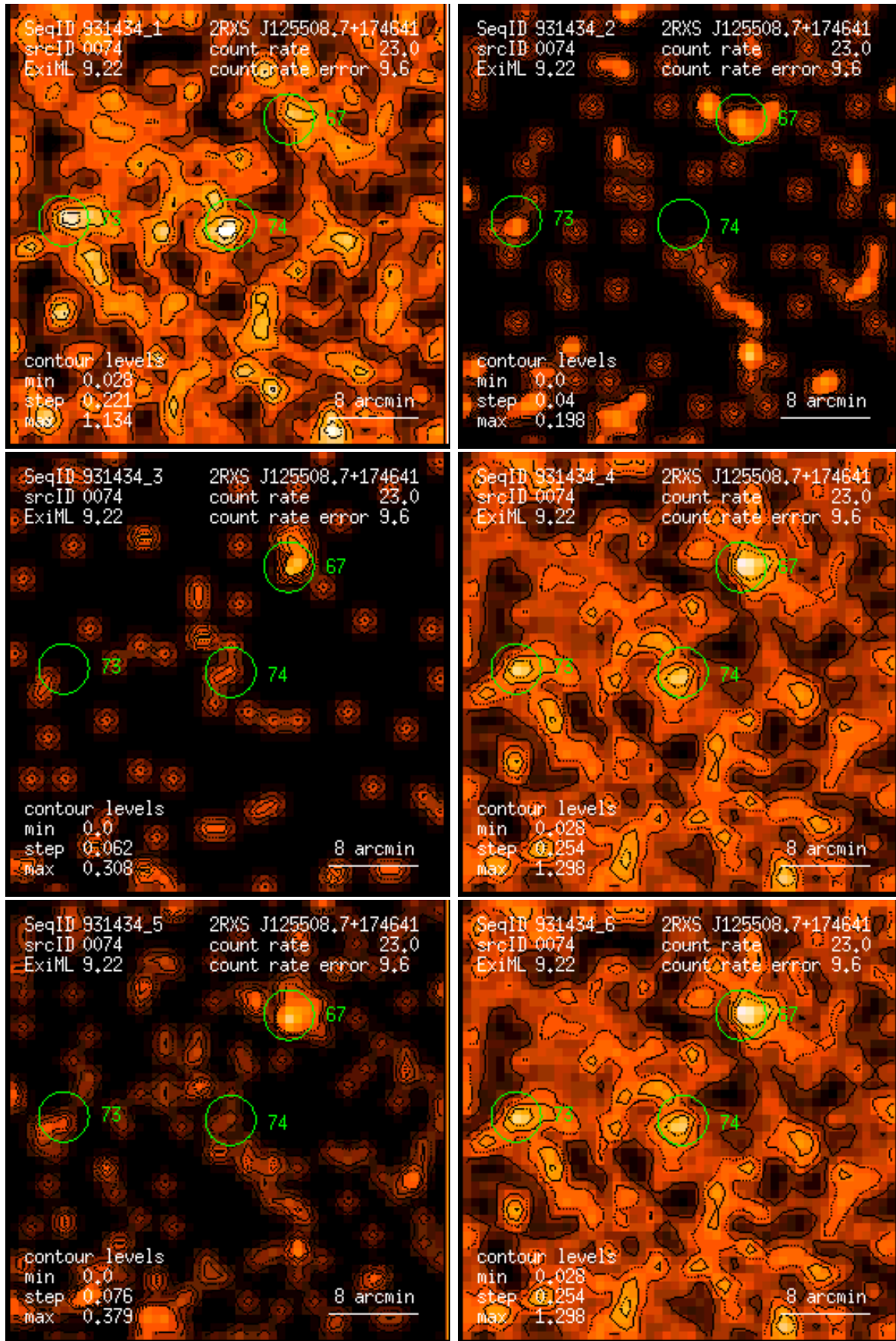
Figure 74: RASS 931434: detection 0074: band rate images, Gaussian filter: (1) PSPC channels 11 – 41, (2) 52 – 90, (3) 91 – 201, (4) 11 – 235, (5) 52 – 201, (6) 11 – 201. Broad band rates in counts/ks. Band rate contour levels in counts/ks/arcmin 2 .
