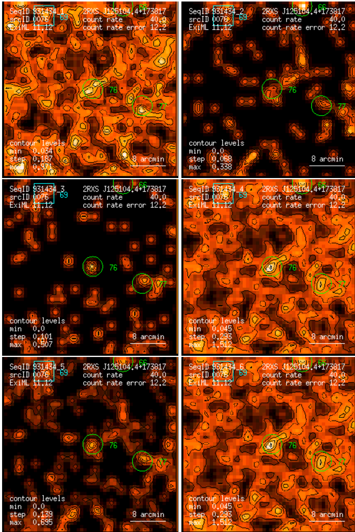
Figure 76: RASS 931434: detection 0076: band rate images, Gaussian filter: (1) PSPC channels 11 – 41, (2) 52 – 90, (3) 91 – 201, (4) 11 – 235, (5) 52 – 201, (6) 11 – 201. Broad band rates in counts/ks. Band rate contour levels in counts/ks/arcmin 2 .
