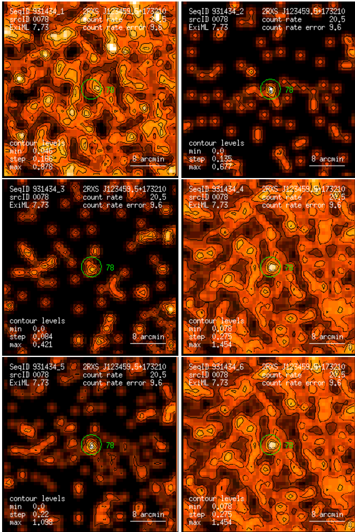
Figure 78: RASS 931434: detection 0078: band rate images, Gaussian filter: (1) PSPC channels 11 – 41, (2) 52 – 90, (3) 91 – 201, (4) 11 – 235, (5) 52 – 201, (6) 11 – 201. Broad band rates in counts/ks. Band rate contour levels in counts/ks/arcmin 2 .
