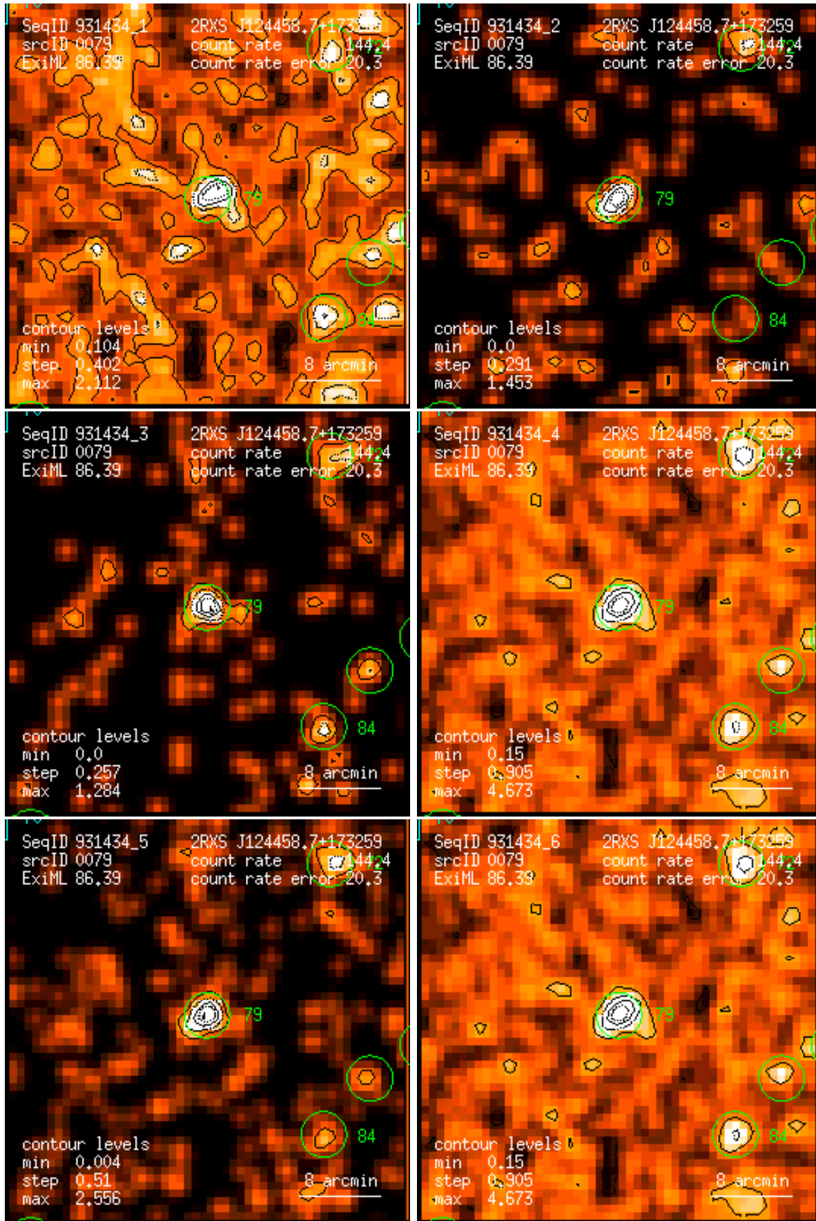
Figure 79: RASS 931434: detection 0079: band rate images, Gaussian filter: (1) PSPC channels 11 – 41, (2) 52 – 90, (3) 91 – 201, (4) 11 – 235, (5) 52 – 201, (6) 11 – 201. Broad band rates in counts/ks. Band rate contour levels in counts/ks/arcmin 2 .
