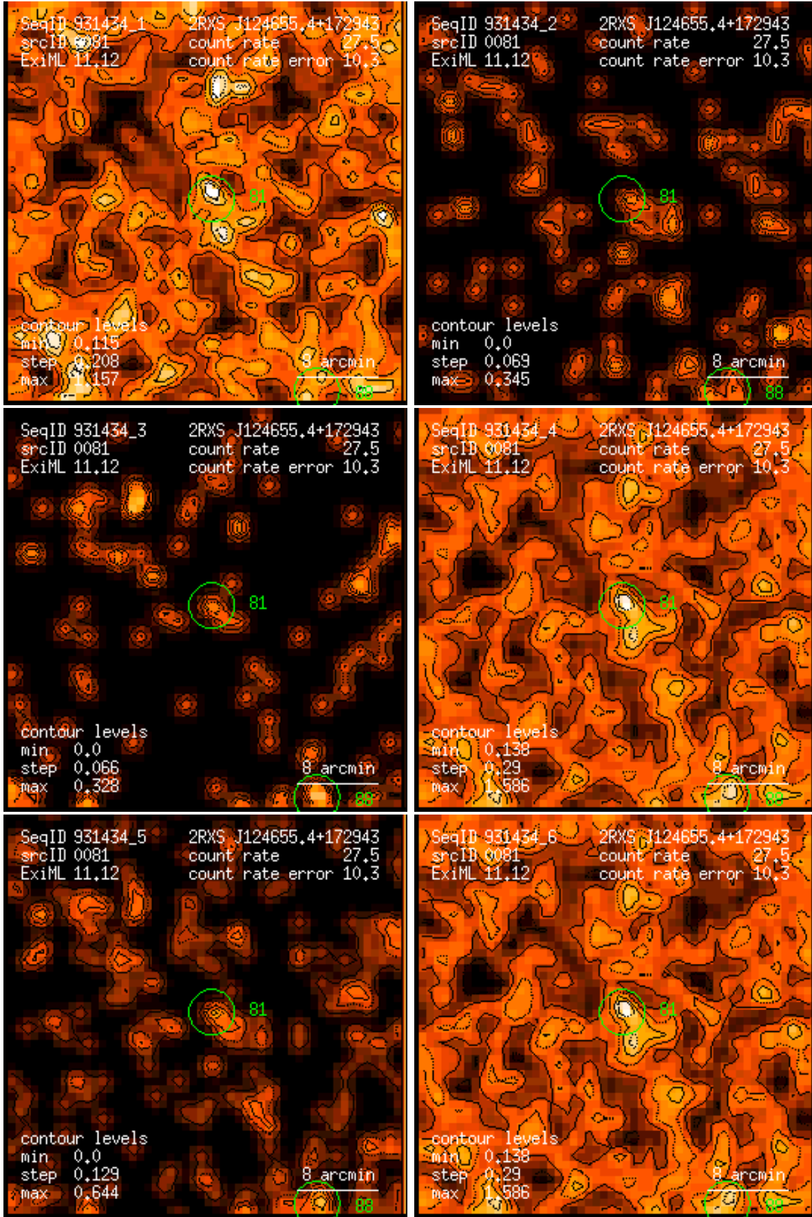
Figure 81: RASS 931434: detection 0081: band rate images, Gaussian filter: (1) PSPC channels 11 – 41, (2) 52 – 90, (3) 91 – 201, (4) 11 – 235, (5) 52 – 201, (6) 11 – 201. Broad band rates in counts/ks. Band rate contour levels in counts/ks/arcmin 2 .
