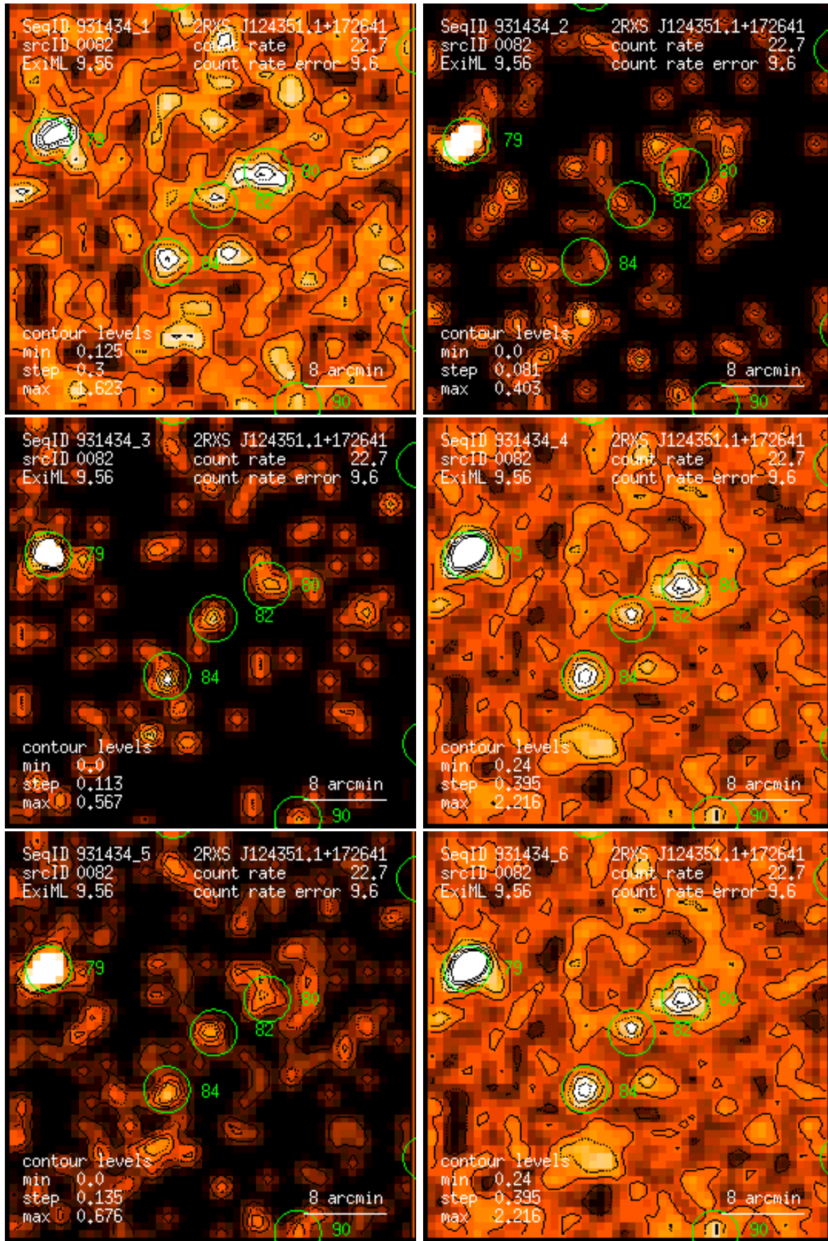
Figure 82: RASS 931434: detection 0082: band rate images, Gaussian filter: (1) PSPC channels 11 – 41, (2) 52 – 90, (3) 91 – 201, (4) 11 – 235, (5) 52 – 201, (6) 11 – 201. Broad band rates in counts/ks. Band rate contour levels in counts/ks/arcmin 2 .
