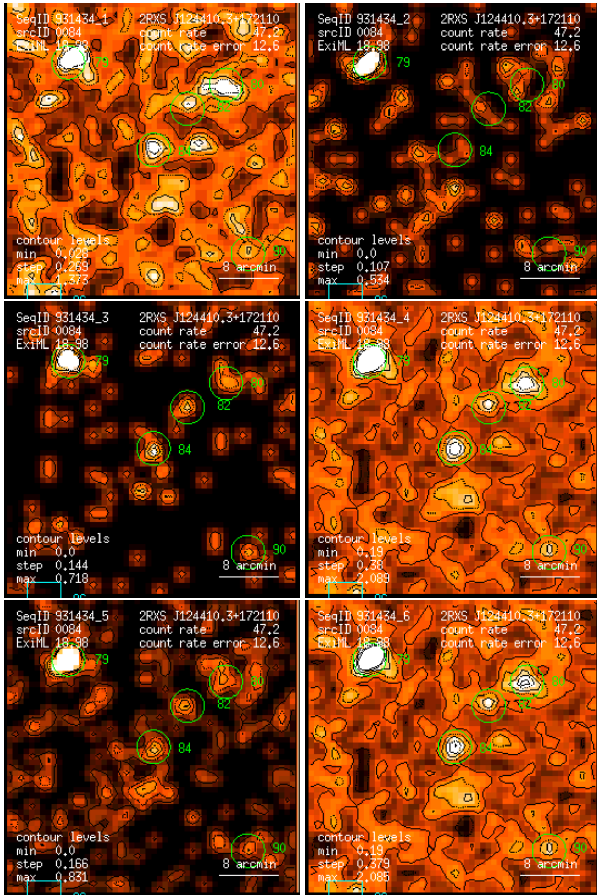
Figure 84: RASS 931434: detection 0084: band rate images, Gaussian filter: (1) PSPC channels 11 – 41, (2) 52 – 90, (3) 91 – 201, (4) 11 – 235, (5) 52 – 201, (6) 11 – 201. Broad band rates in counts/ks. Band rate contour levels in counts/ks/arcmin 2 .
