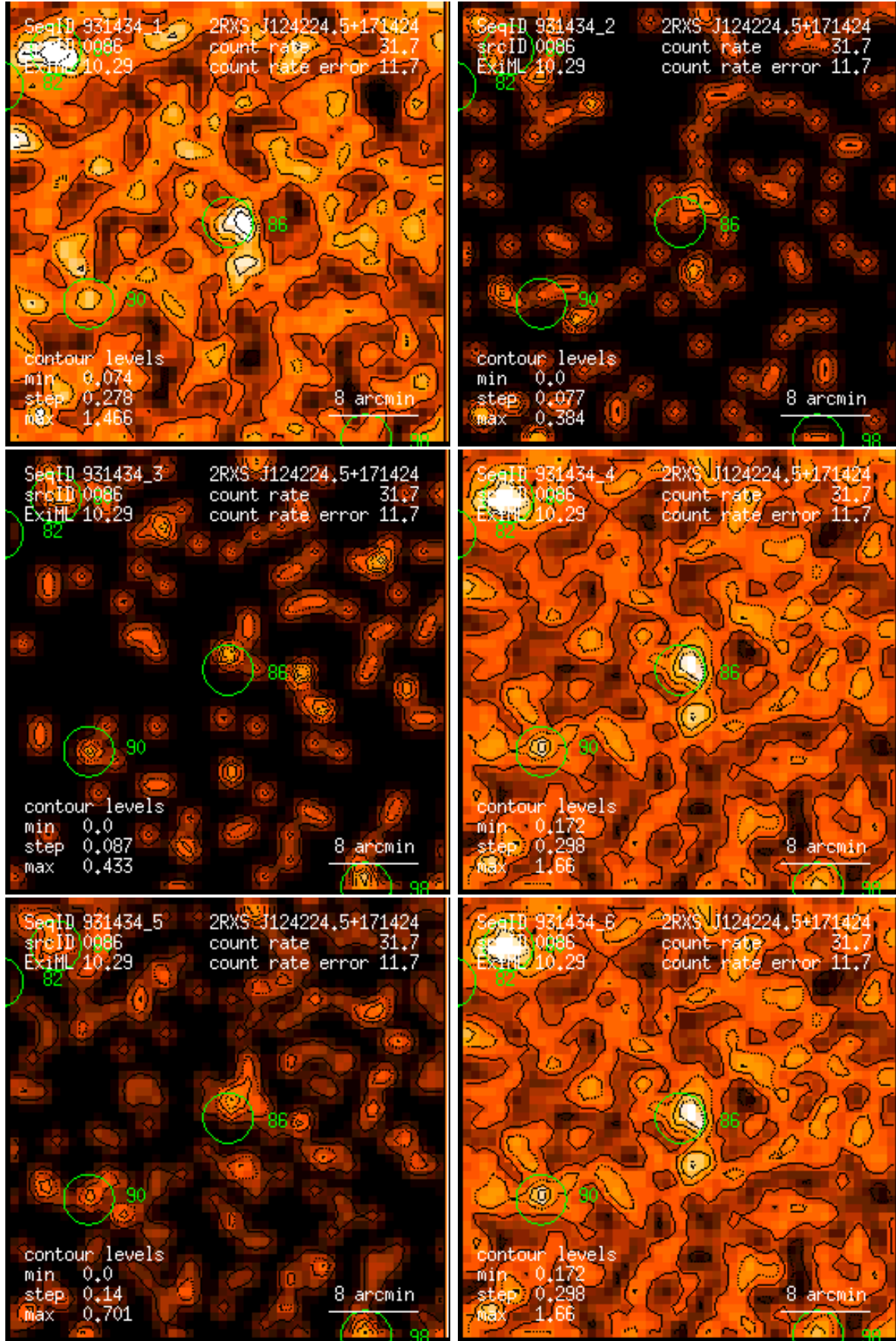
Figure 86: RASS 931434: detection 0086: band rate images, Gaussian filter: (1) PSPC channels 11 – 41, (2) 52 – 90, (3) 91 – 201, (4) 11 – 235, (5) 52 – 201, (6) 11 – 201. Broad band rates in counts/ks. Band rate contour levels in counts/ks/arcmin 2 .
