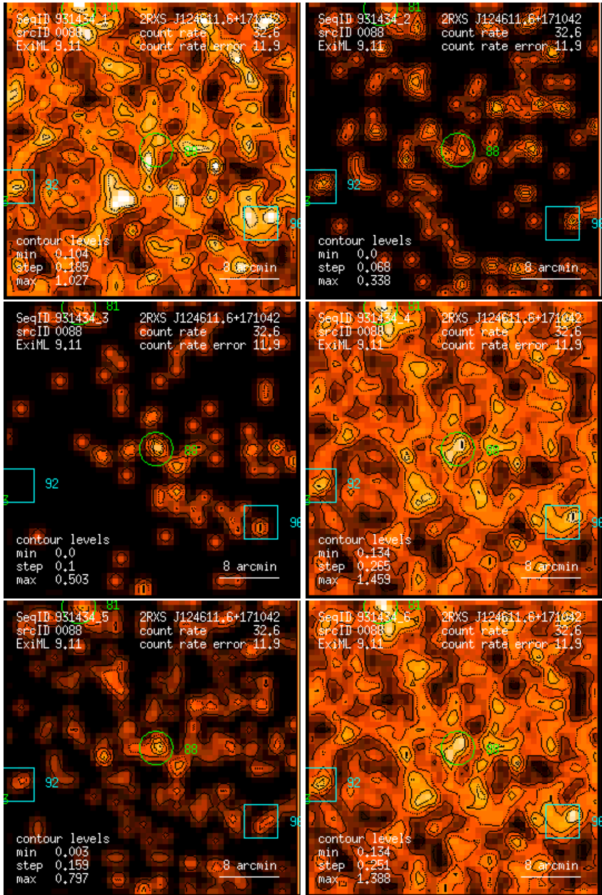
Figure 88: RASS 931434: detection 0088: band rate images, Gaussian filter: (1) PSPC channels 11 – 41, (2) 52 – 90, (3) 91 – 201, (4) 11 – 235, (5) 52 – 201, (6) 11 – 201. Broad band rates in counts/ks. Band rate contour levels in counts/ks/arcmin 2 .
