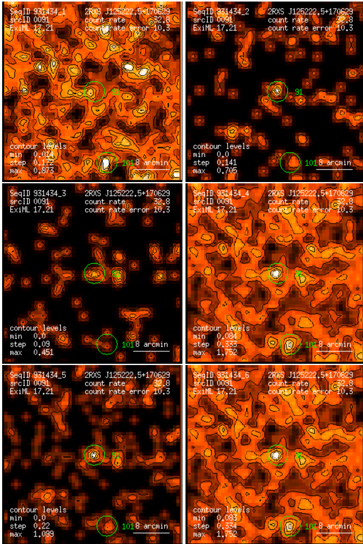
Figure 91: RASS 931434: detection 0091: band rate images, Gaussian filter: (1) PSPC channels 11 – 41, (2) 52 – 90, (3) 91 – 201, (4) 11 – 235, (5) 52 – 201, (6) 11 – 201. Broad band rates in counts/ks. Band rate contour levels in counts/ks/arcmin 2 .
