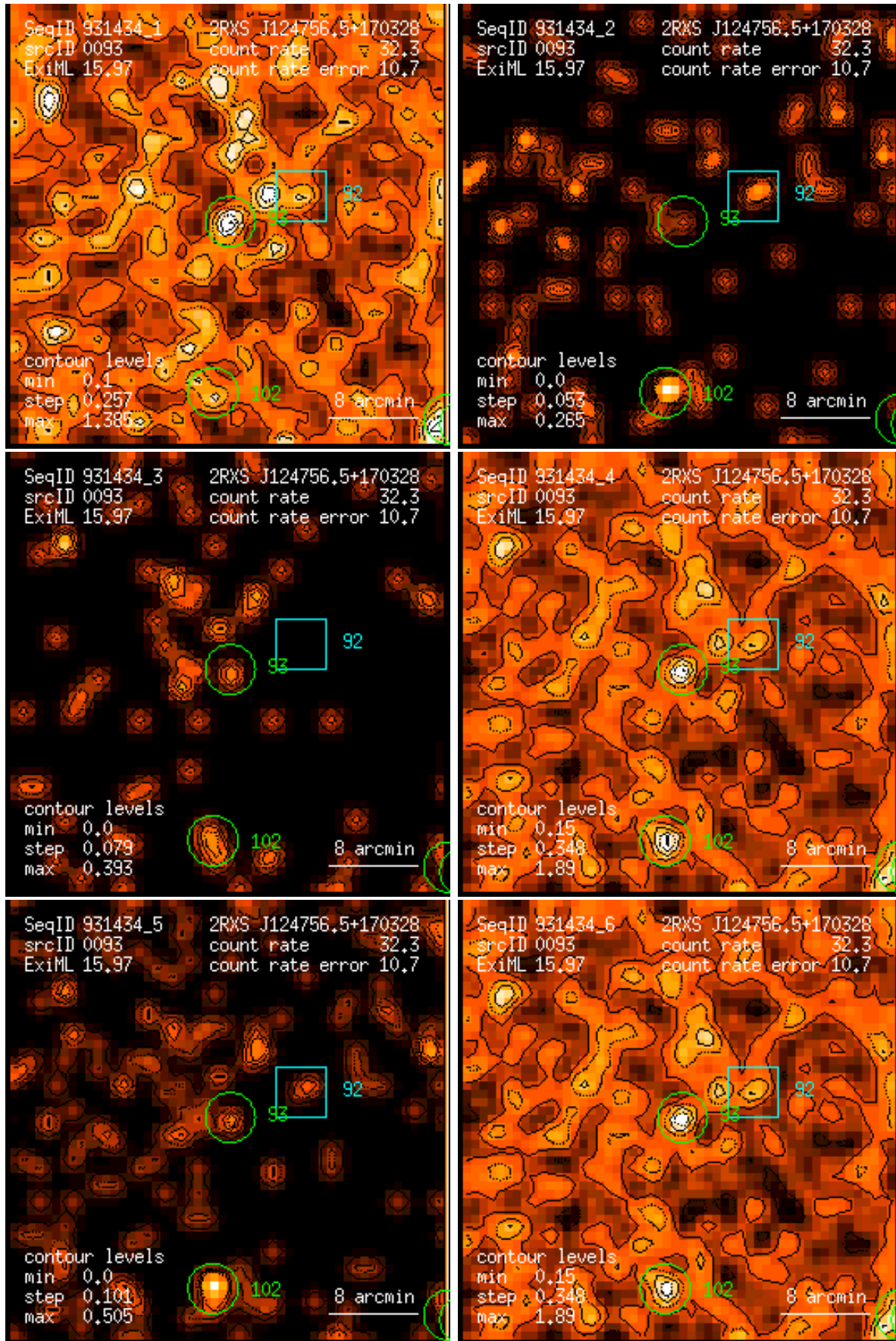
Figure 93: RASS 931434: detection 0093: band rate images, Gaussian filter: (1) PSPC channels 11 – 41, (2) 52 – 90, (3) 91 – 201, (4) 11 – 235, (5) 52 – 201, (6) 11 – 201. Broad band rates in counts/ks. Band rate contour levels in counts/ks/arcmin 2 .
