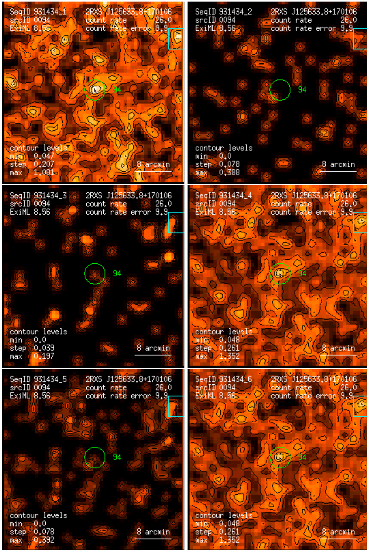
Figure 94: RASS 931434: detection 0094: band rate images, Gaussian filter: (1) PSPC channels 11 – 41, (2) 52 – 90, (3) 91 – 201, (4) 11 – 235, (5) 52 – 201, (6) 11 – 201. Broad band rates in counts/ks. Band rate contour levels in counts/ks/arcmin 2 .
