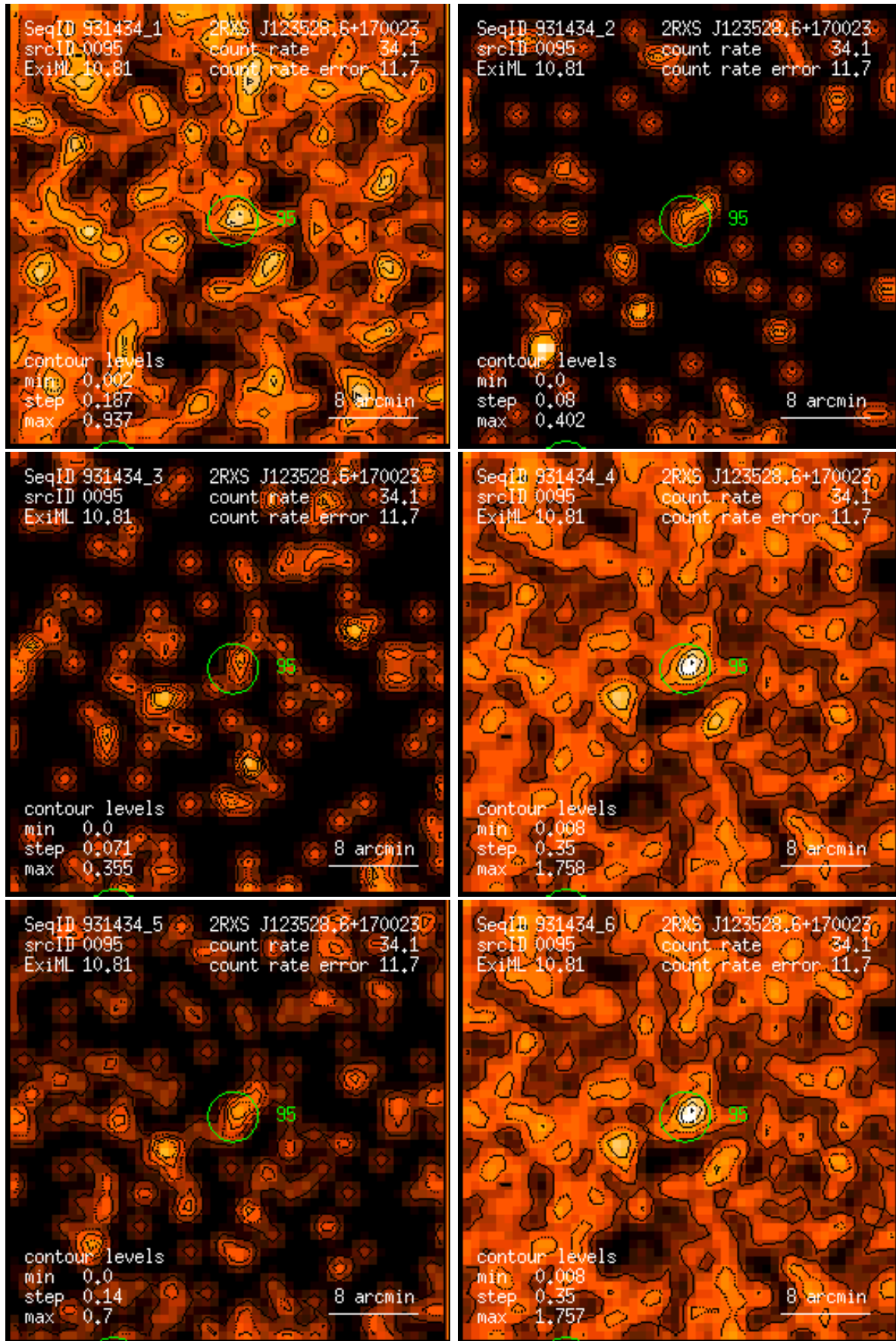
Figure 95: RASS 931434: detection 0095: band rate images, Gaussian filter: (1) PSPC channels 11 – 41, (2) 52 – 90, (3) 91 – 201, (4) 11 – 235, (5) 52 – 201, (6) 11 – 201. Broad band rates in counts/ks. Band rate contour levels in counts/ks/arcmin 2 .
