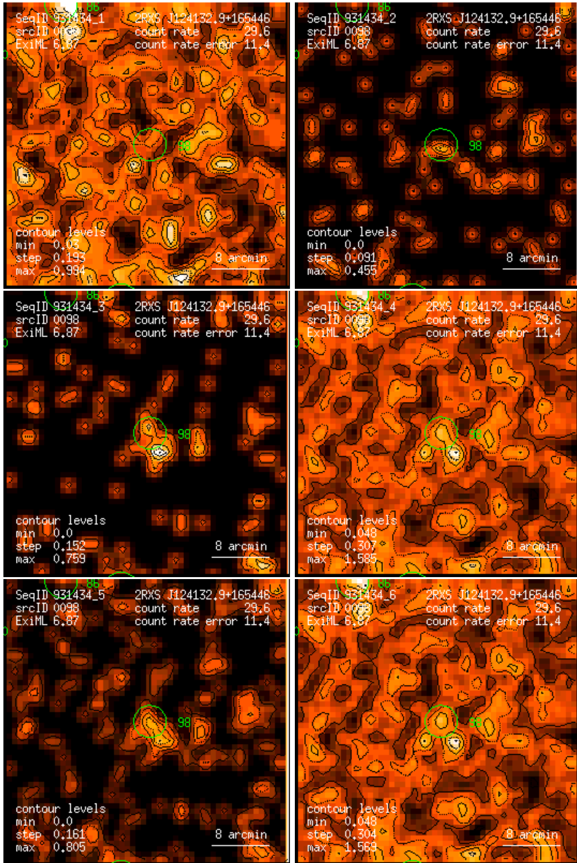
Figure 98: RASS 931434: detection 0098: band rate images, Gaussian filter: (1) PSPC channels 11 – 41, (2) 52 – 90, (3) 91 – 201, (4) 11 – 235, (5) 52 – 201, (6) 11 – 201. Broad band rates in counts/ks. Band rate contour levels in counts/ks/arcmin 2 .
