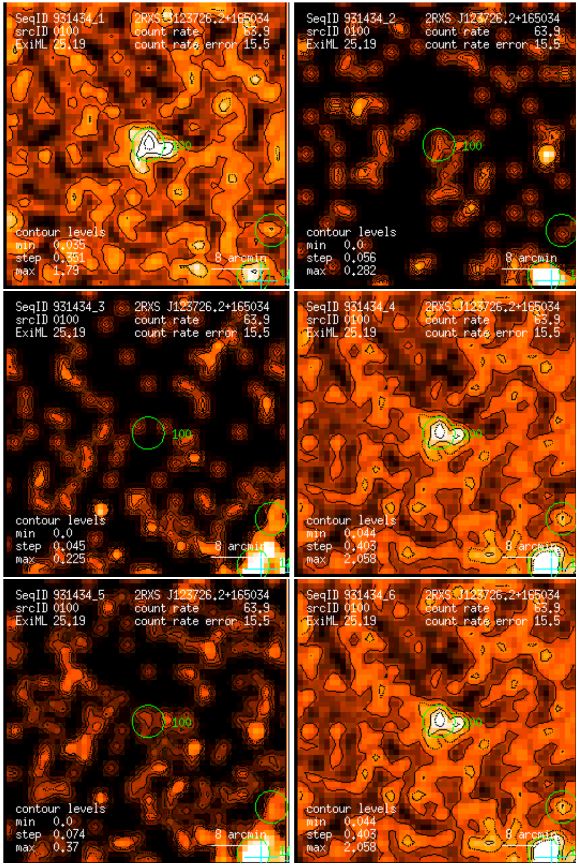
Figure 100: RASS 931434: detection 0100: band rate images, Gaussian filter: (1) PSPC channels 11 – 41, (2) 52 – 90, (3) 91 – 201, (4) 11 – 235, (5) 52 – 201, (6) 11 – 201. Broad band rates in counts/ks. Band rate contour levels in counts/ks/arcmin 2 .
