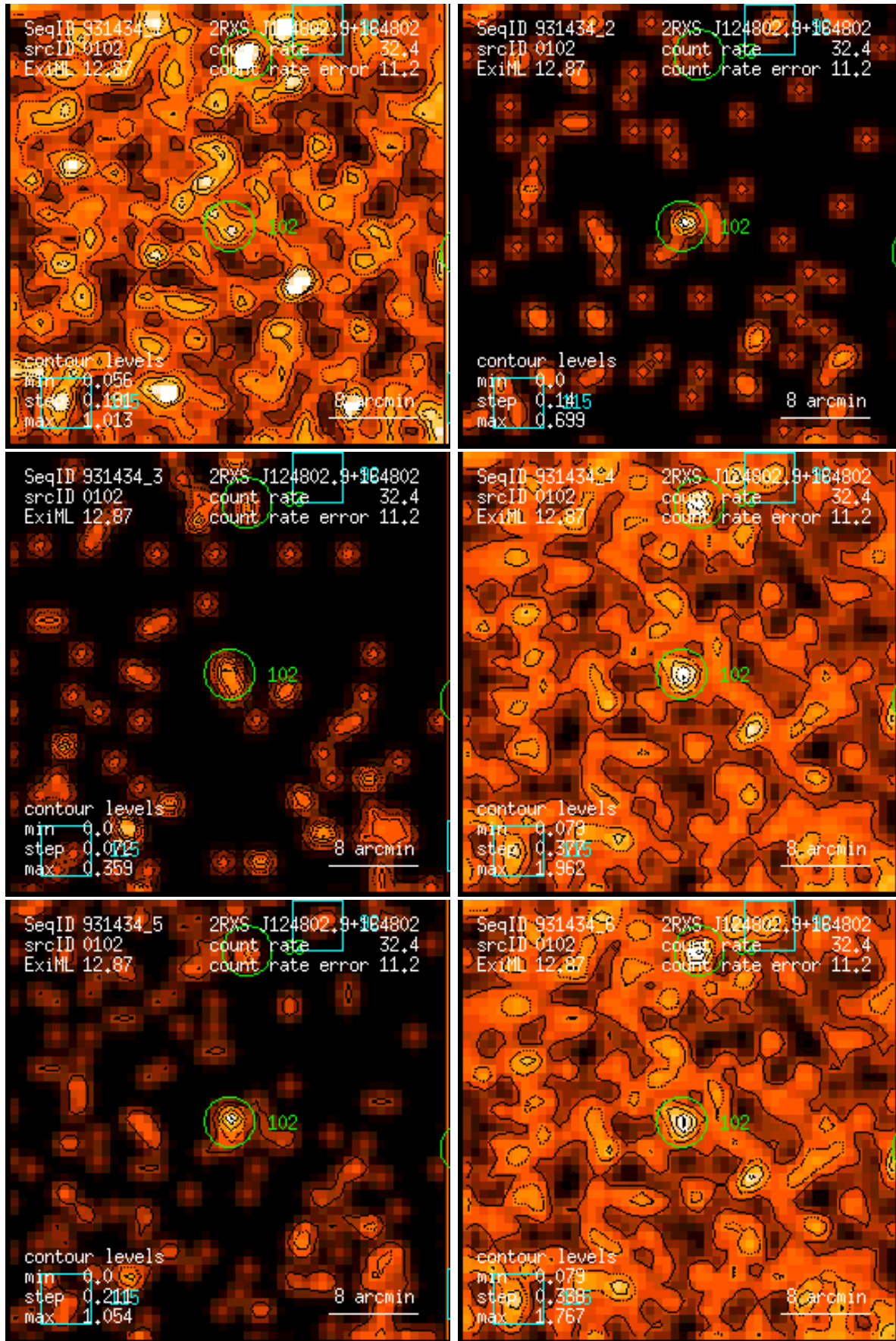
Figure 102: RASS 931434: detection 0102: band rate images, Gaussian filter: (1) PSPC channels 11 – 41, (2) 52 – 90, (3) 91 – 201, (4) 11 – 235, (5) 52 – 201, (6) 11 – 201. Broad band rates in counts/ks. Band rate contour levels in counts/ks/arcmin 2 .
