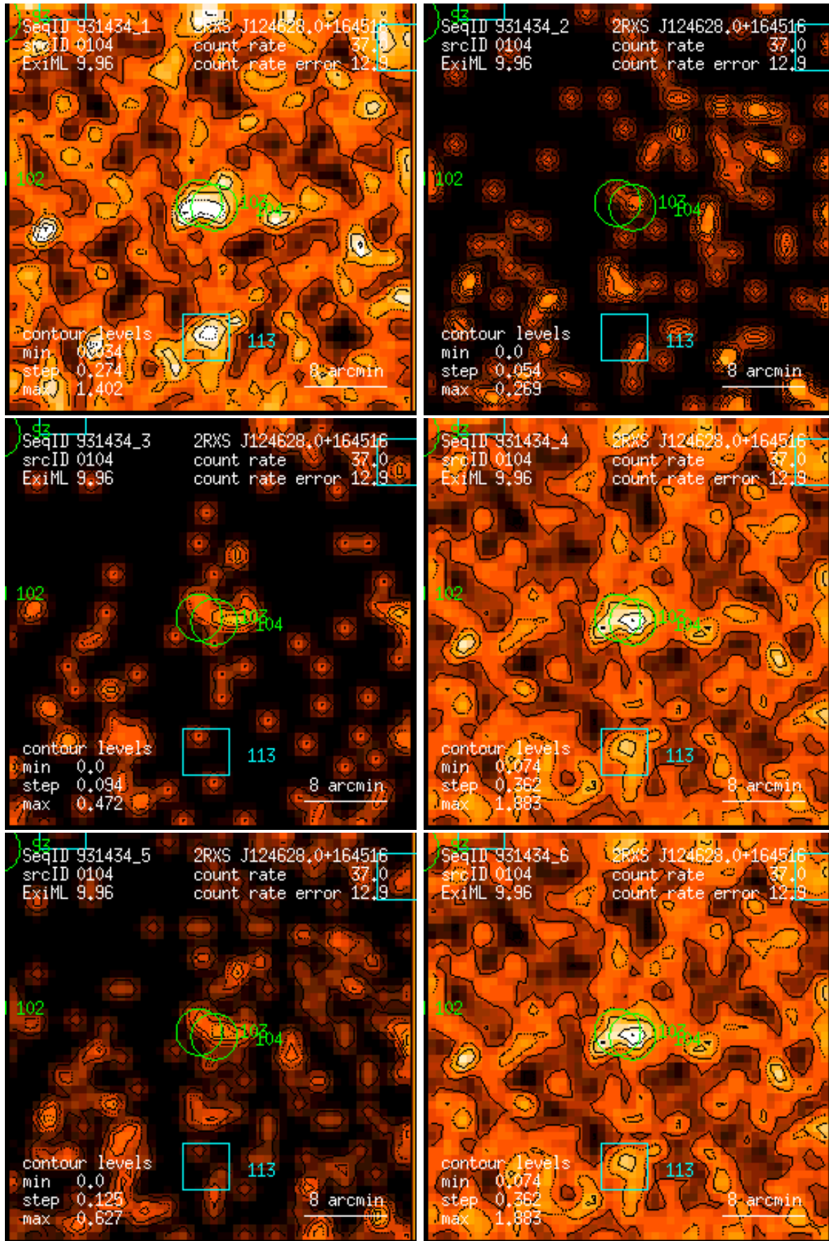
Figure 104: RASS 931434: detection 0104: band rate images, Gaussian filter: (1) PSPC channels 11 – 41, (2) 52 – 90, (3) 91 – 201, (4) 11 – 235, (5) 52 – 201, (6) 11 – 201. Broad band rates in counts/ks. Band rate contour levels in counts/ks/arcmin 2 .
