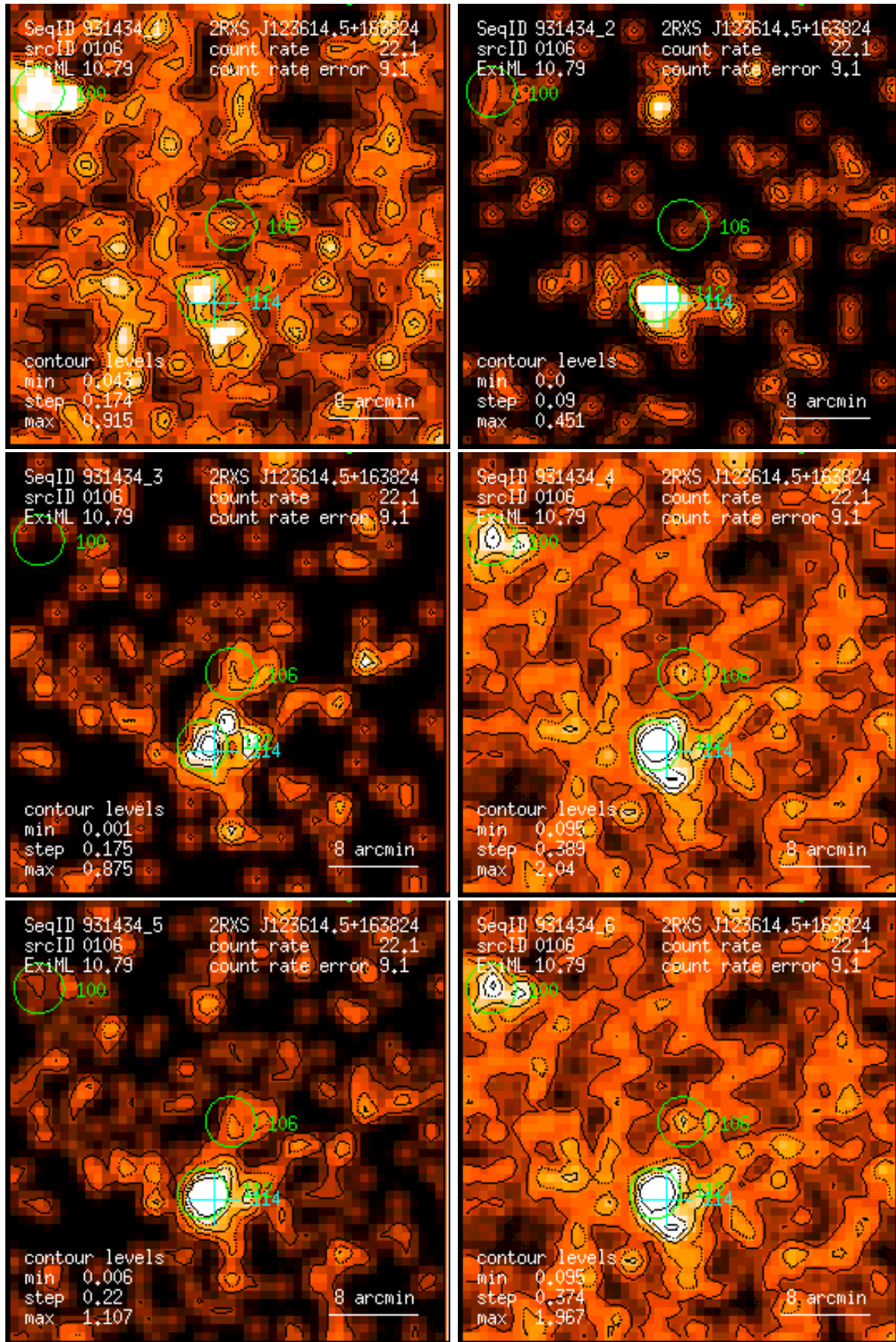
Figure 106: RASS 931434: detection 0106: band rate images, Gaussian filter: (1) PSPC channels 11 – 41, (2) 52 – 90, (3) 91 – 201, (4) 11 – 235, (5) 52 – 201, (6) 11 – 201. Broad band rates in counts/ks. Band rate contour levels in counts/ks/arcmin 2 .
