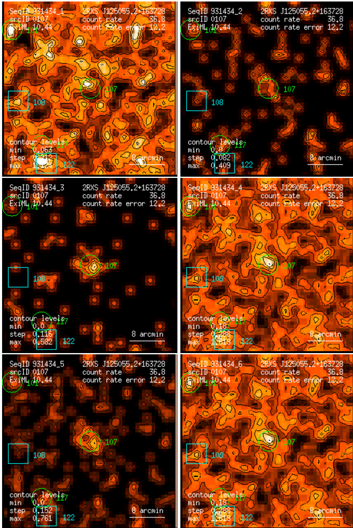
Figure 107: RASS 931434: detection 0107: band rate images, Gaussian filter: (1) PSPC channels 11 – 41, (2) 52 – 90, (3) 91 – 201, (4) 11 – 235, (5) 52 – 201, (6) 11 – 201. Broad band rates in counts/ks. Band rate contour levels in counts/ks/arcmin 2 .
