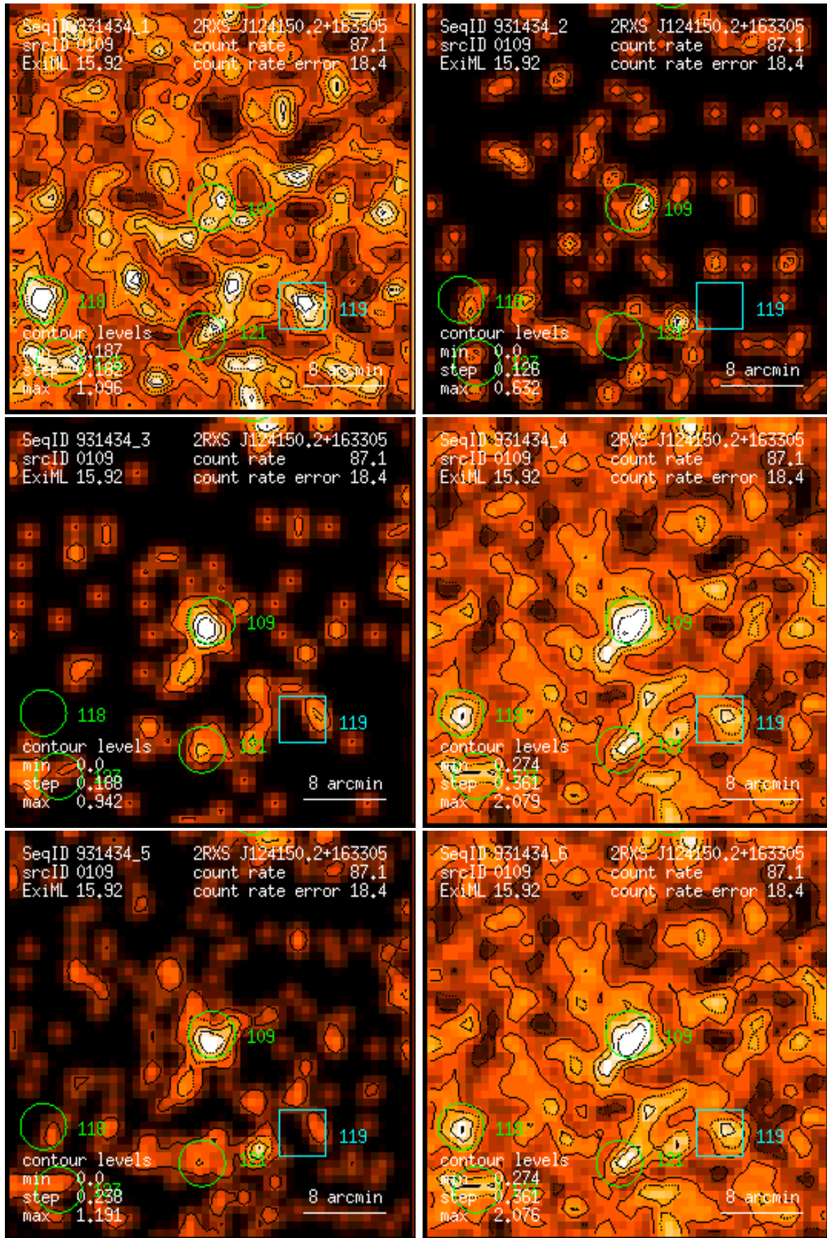
Figure 109: RASS 931434: detection 0109: band rate images, Gaussian filter: (1) PSPC channels 11 – 41, (2) 52 – 90, (3) 91 – 201, (4) 11 – 235, (5) 52 – 201, (6) 11 – 201. Broad band rates in counts/ks. Band rate contour levels in counts/ks/arcmin 2 .
