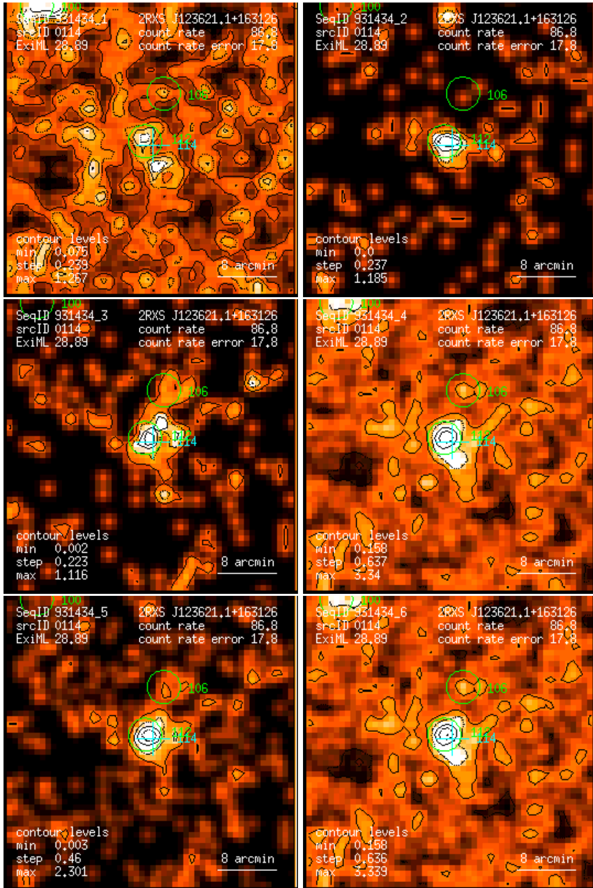
Figure 114: RASS 931434: detection 0114: band rate images, Gaussian filter: (1) PSPC channels 11 – 41, (2) 52 – 90, (3) 91 – 201, (4) 11 – 235, (5) 52 – 201, (6) 11 – 201. Broad band rates in counts/ks. Band rate contour levels in counts/ks/arcmin 2 .
