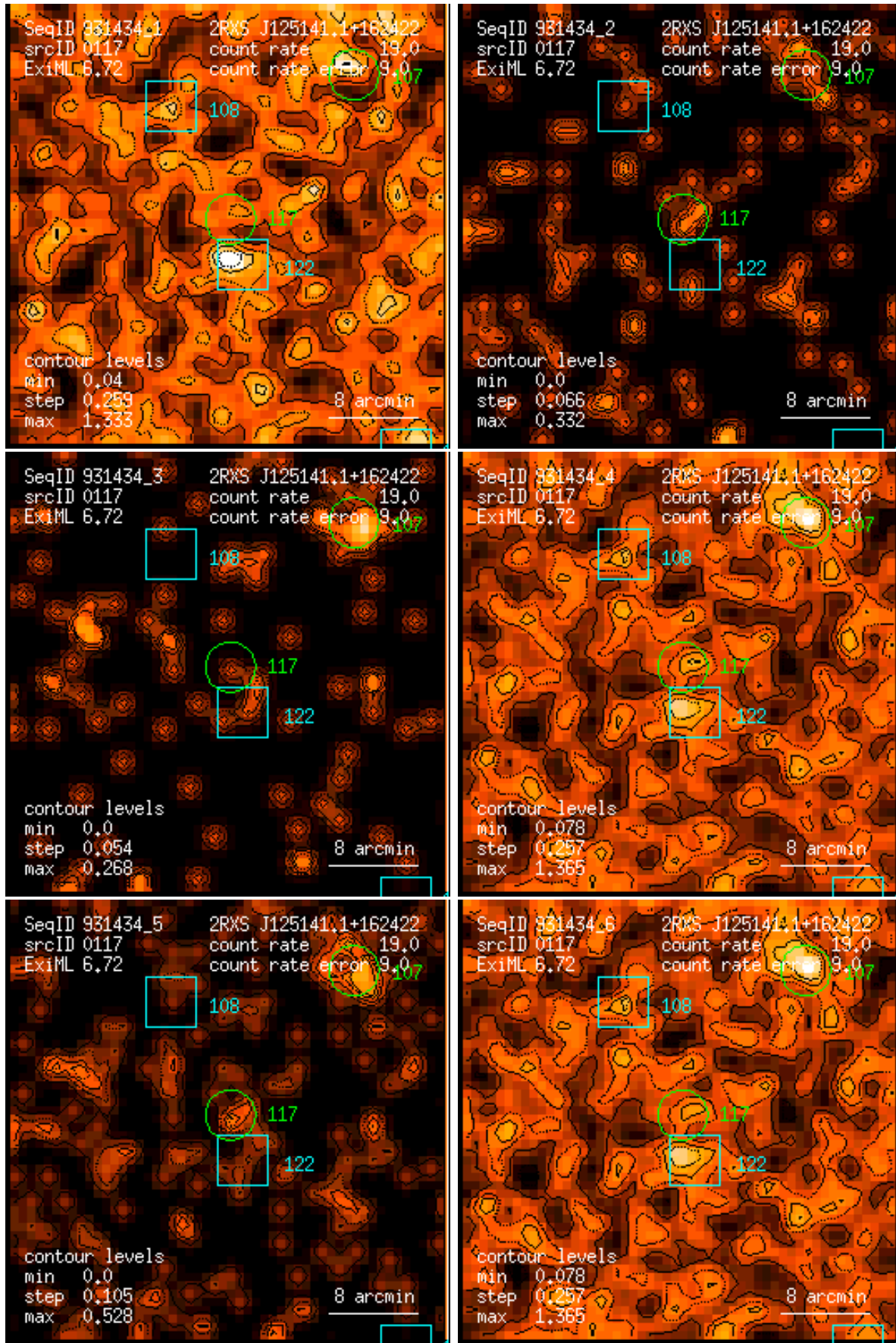
Figure 117: RASS 931434: detection 0117: band rate images, Gaussian filter: (1) PSPC channels 11 – 41, (2) 52 – 90, (3) 91 – 201, (4) 11 – 235, (5) 52 – 201, (6) 11 – 201. Broad band rates in counts/ks. Band rate contour levels in counts/ks/arcmin 2 .
