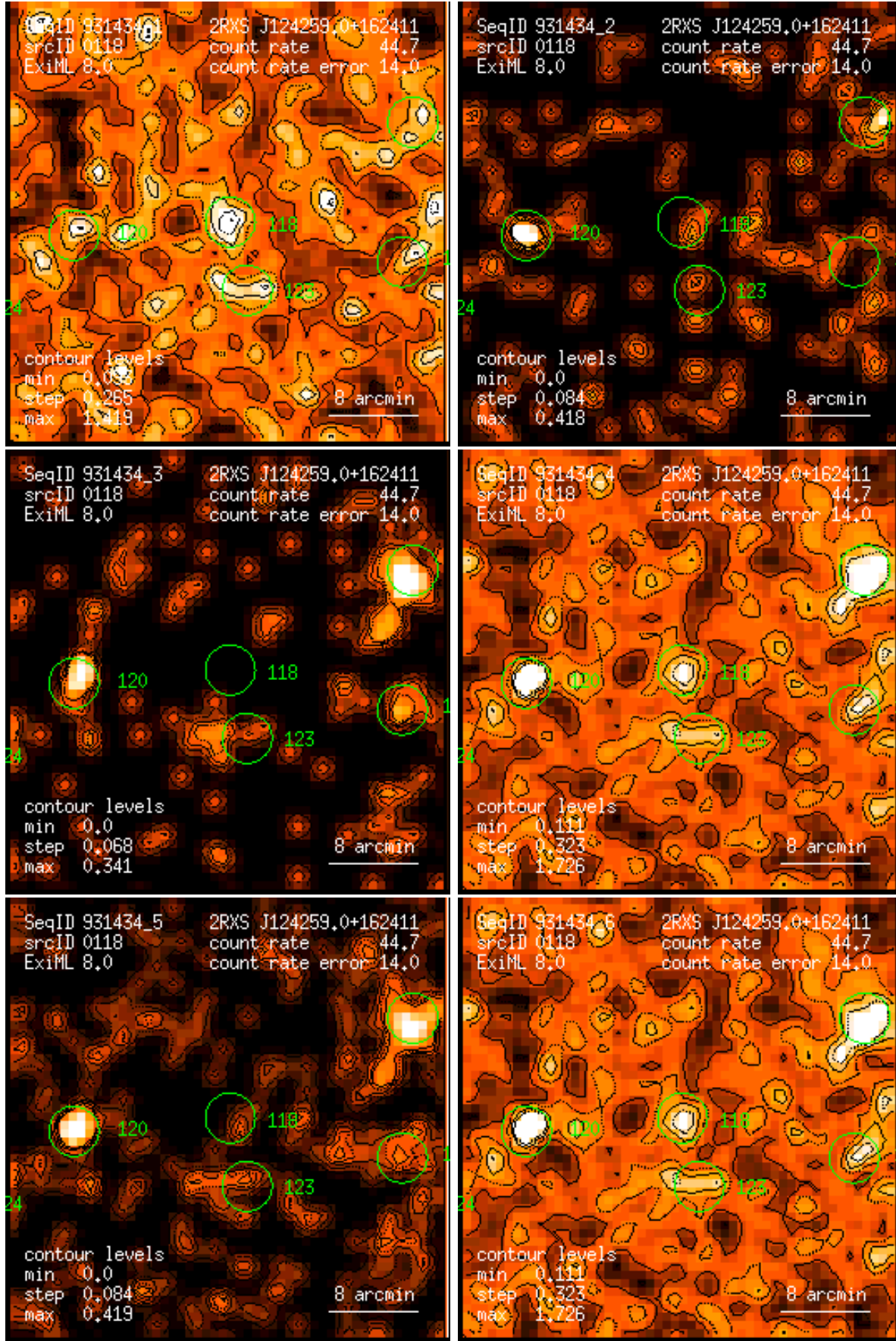
Figure 118: RASS 931434: detection 0118: band rate images, Gaussian filter: (1) PSPC channels 11 – 41, (2) 52 – 90, (3) 91 – 201, (4) 11 – 235, (5) 52 – 201, (6) 11 – 201. Broad band rates in counts/ks. Band rate contour levels in counts/ks/arcmin 2 .
