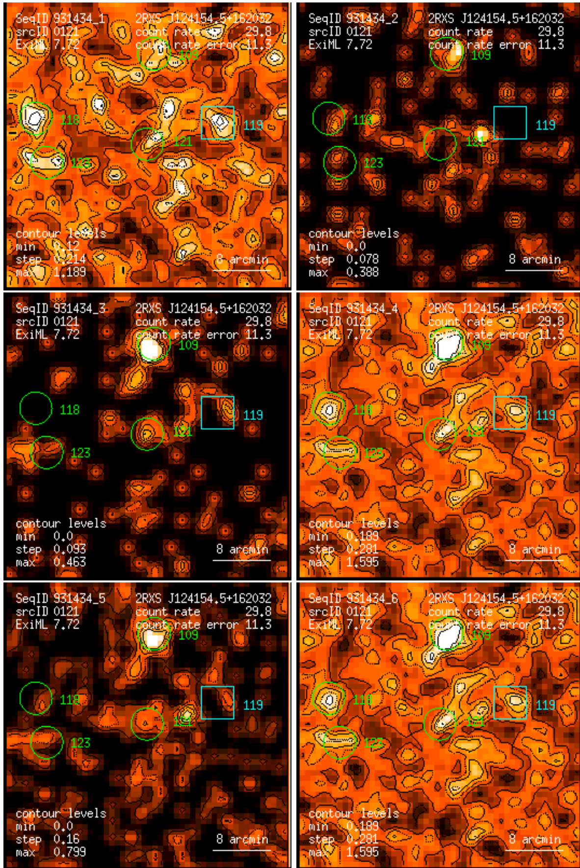
Figure 121: RASS 931434: detection 0121: band rate images, Gaussian filter: (1) PSPC channels 11 – 41, (2) 52 – 90, (3) 91 – 201, (4) 11 – 235, (5) 52 – 201, (6) 11 – 201. Broad band rates in counts/ks. Band rate contour levels in counts/ks/arcmin 2 .
